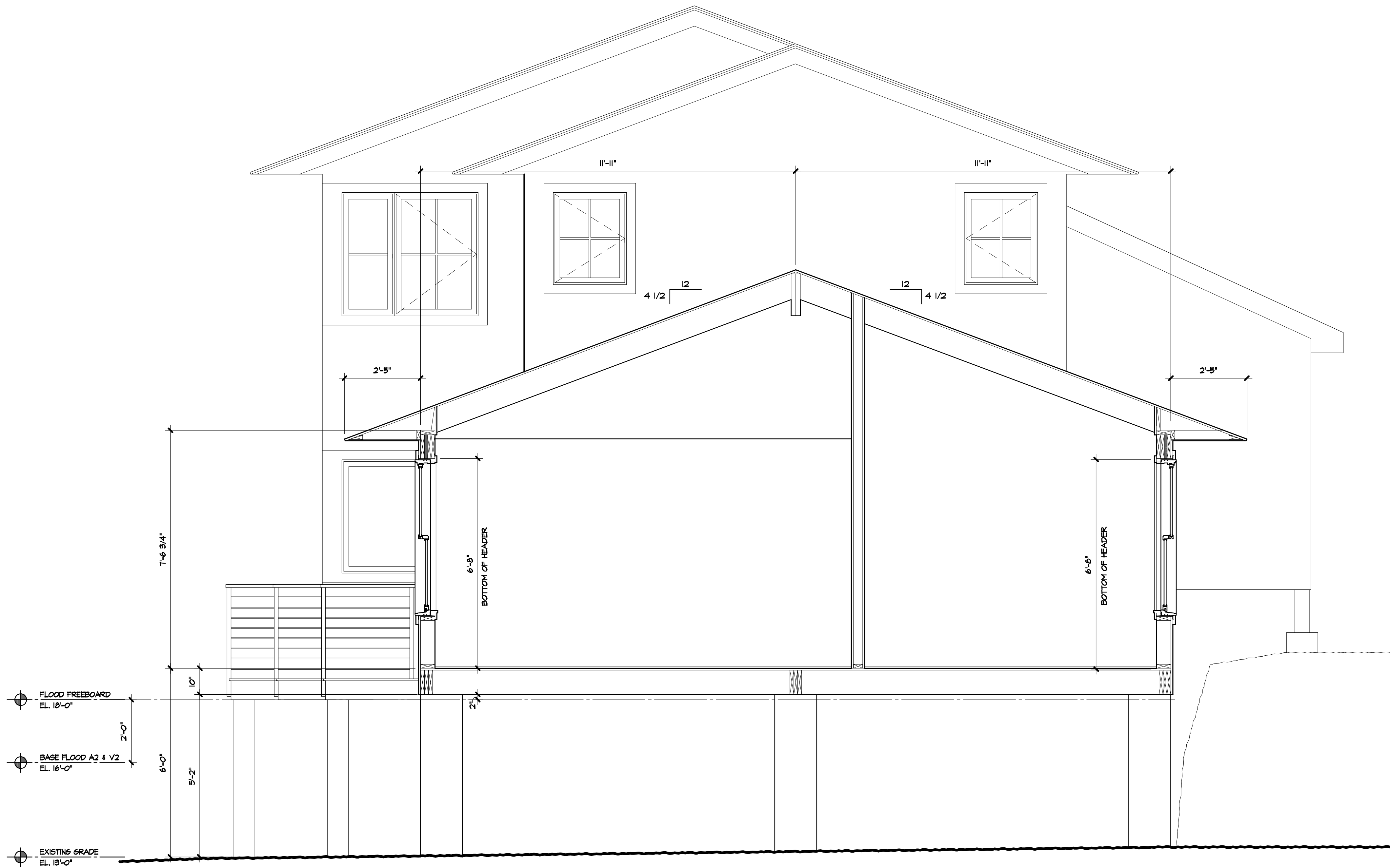
1 CROSS-SECTION A3.3 1/2" = 1'-0"
