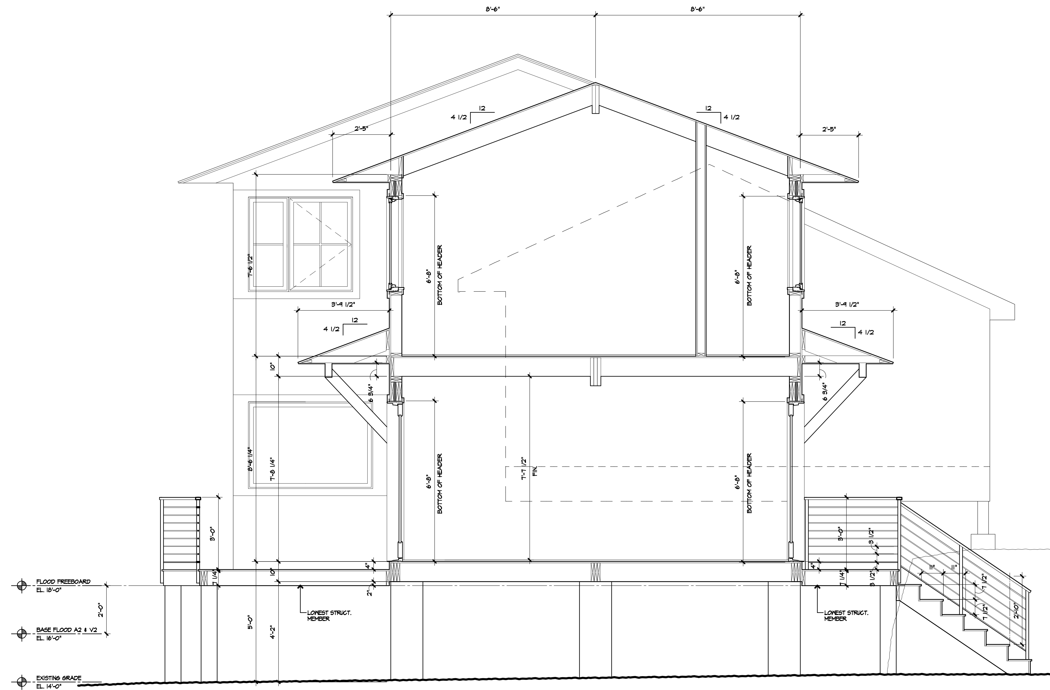
1 CROSS-SECTION A3.2 1/2" = 1'-0"
