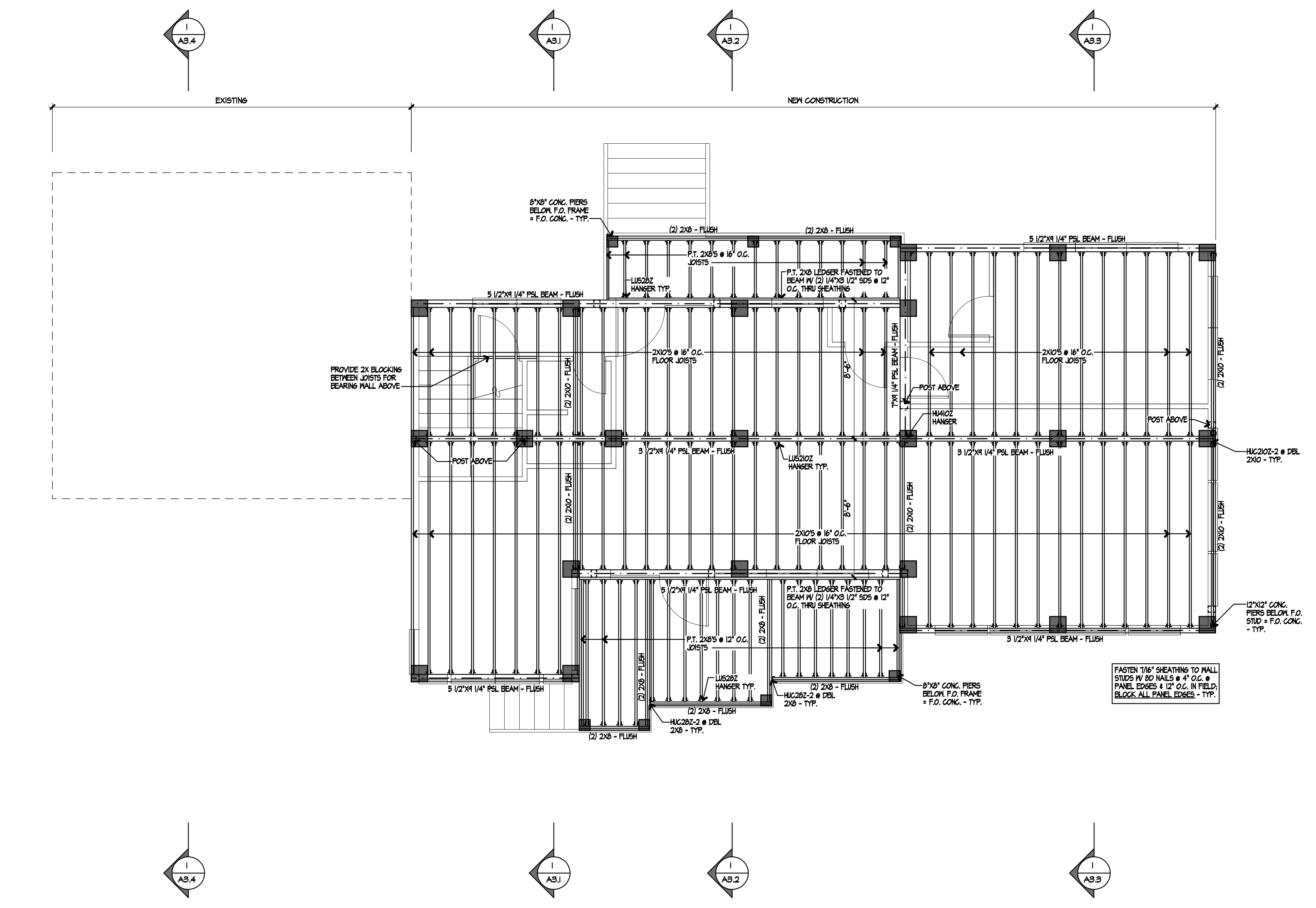
1 FIRST FRAMING FLOOR PLAN S1.2 1/4" = 1'-0"
