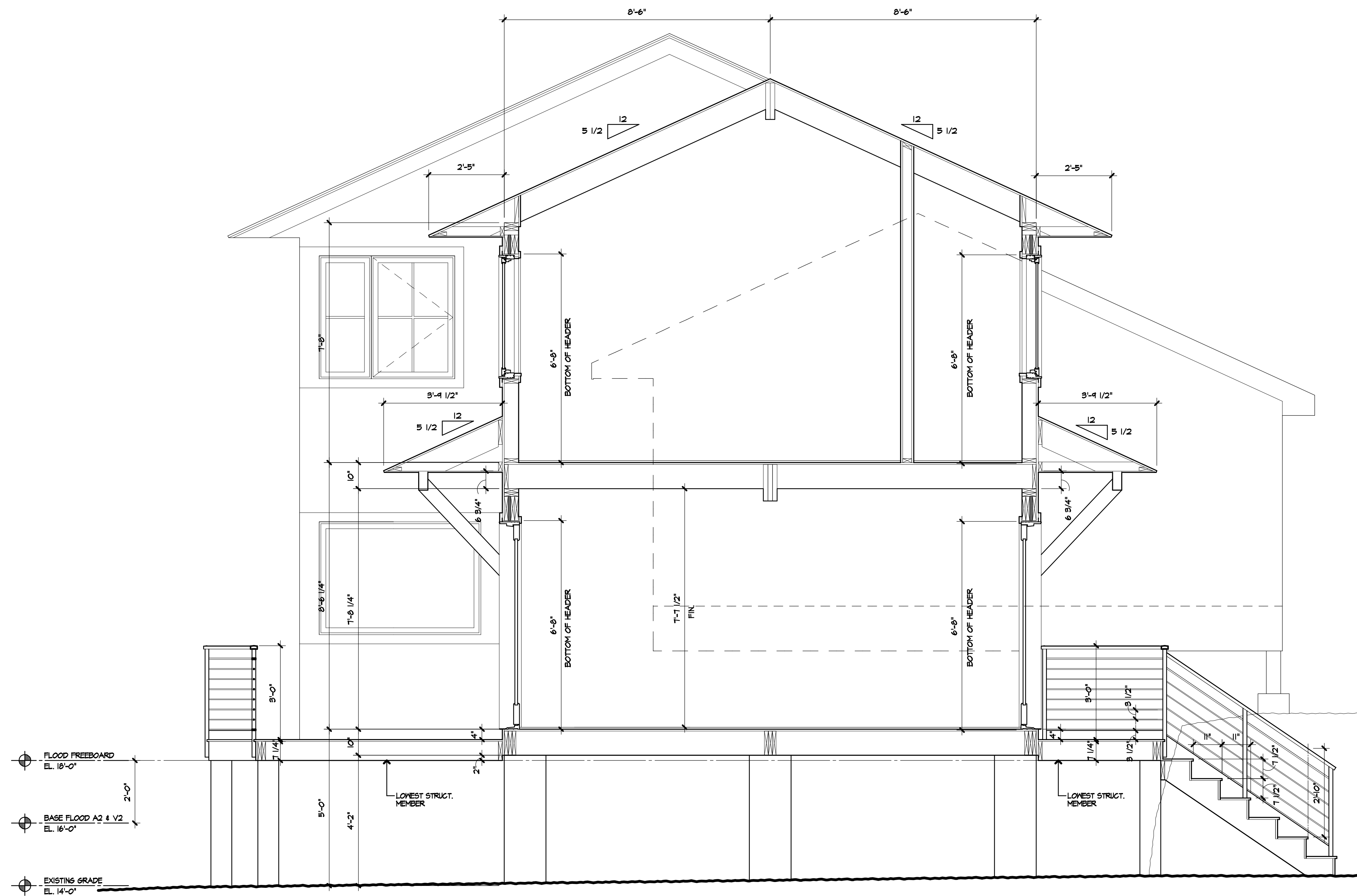
1 CROSS-SECTION A3.2 1/2" = 1'-0"
