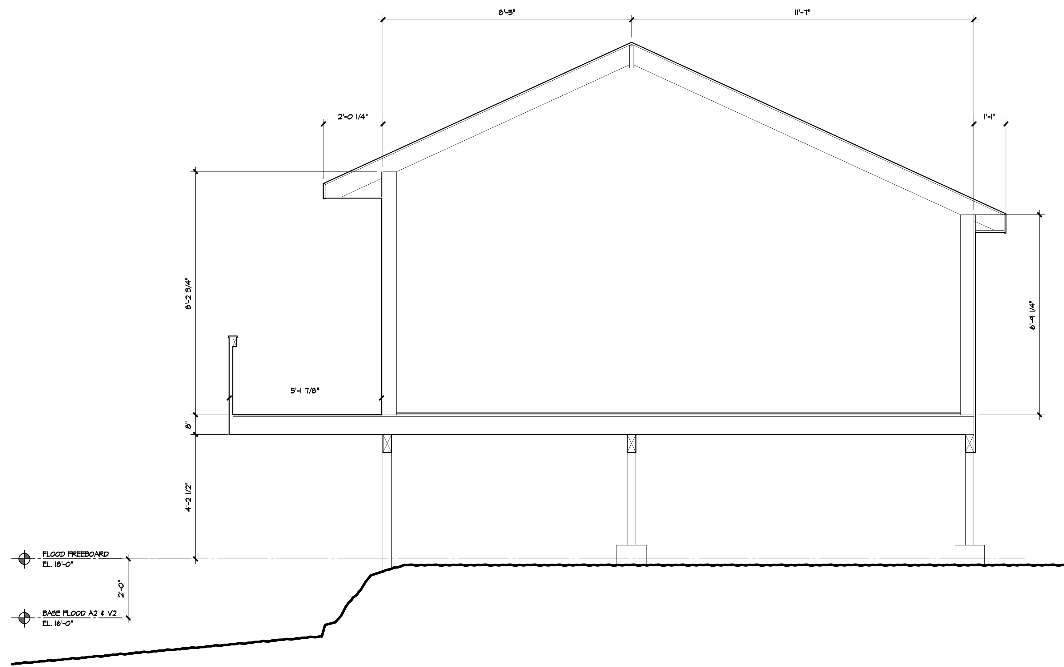
1 A3.4 EXISTING CROSS-SECTION 1/2" = 1'-0"
