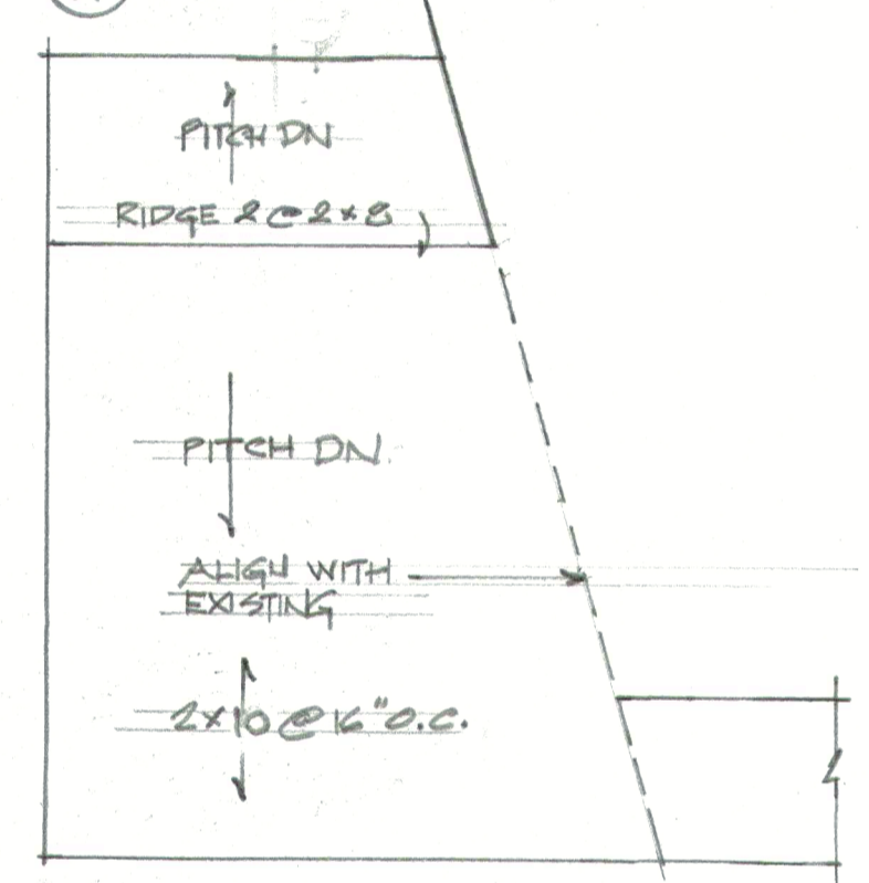
2 ROOF FRAMING 4
