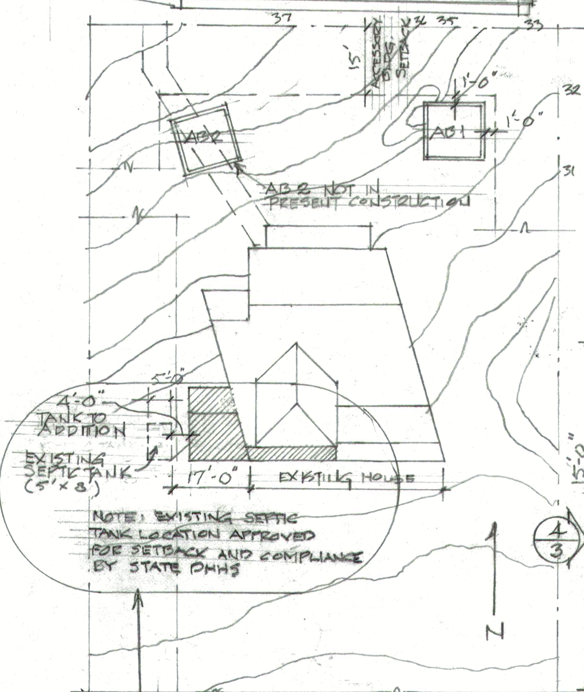
3 SITE PLAN 3 1:20 REVISED 10.24.17
