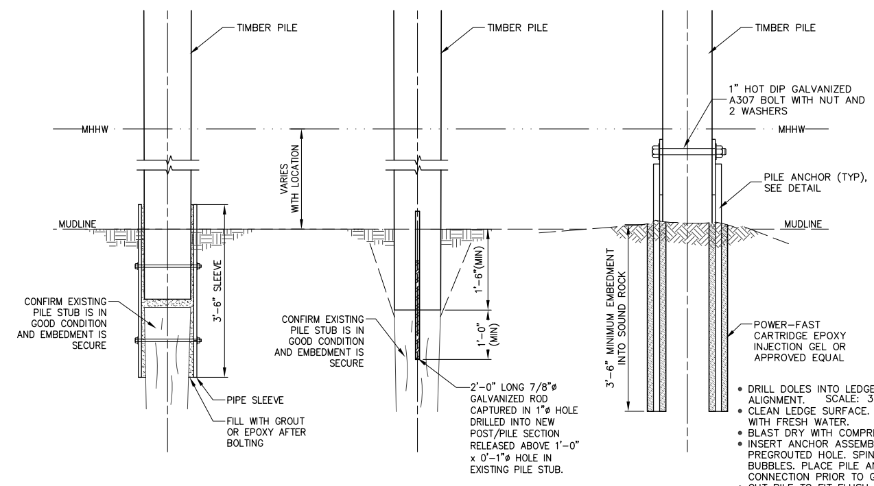
SLEEVED PILE OPTION PINNED PILE OPTION PILE ANCHOR
