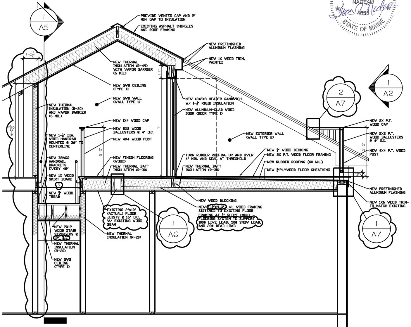
1. BUILDING SECTION
