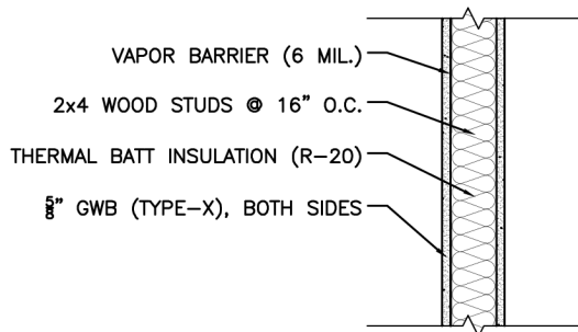
WALL TYPE 1
