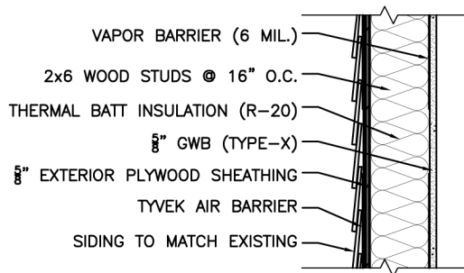
WALL TYPE 2
