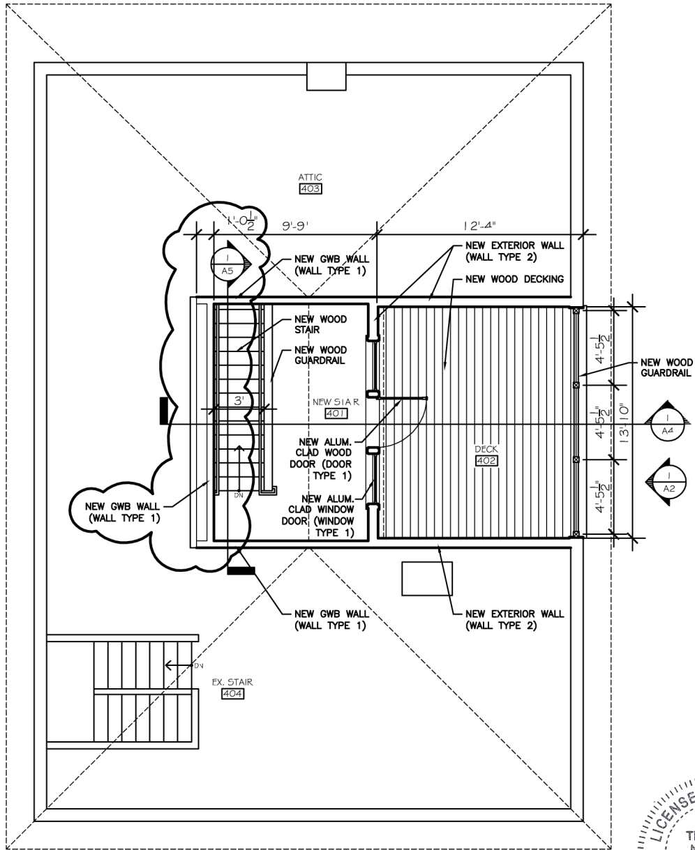
1. PROPOSED ROOF PLAN
