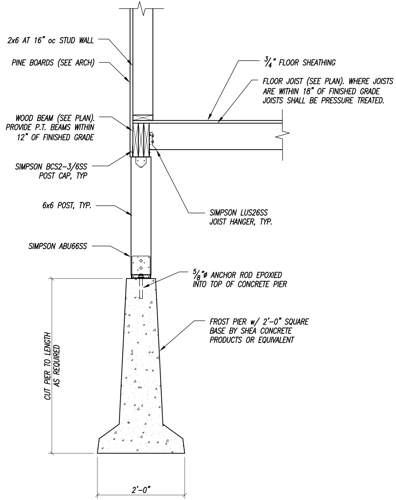
1 SECTION 3/4" = 1'-0"
