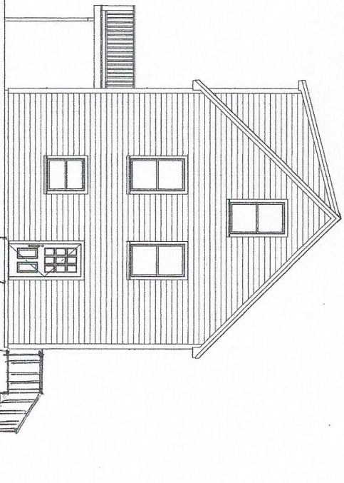
LEFT ELEVATION
