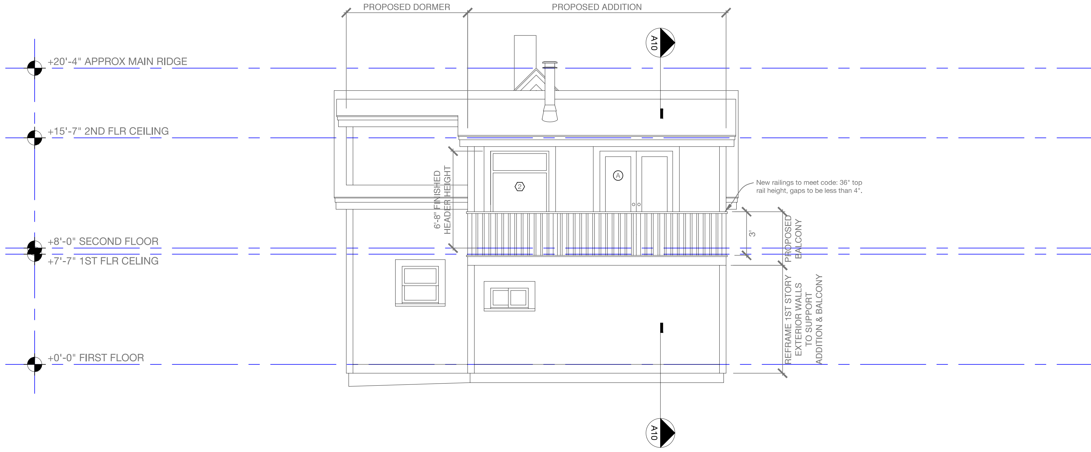
A Proposed East Elevation:
