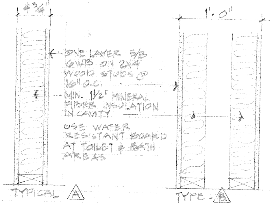
PARTITION TYPES
