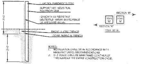
1 PREFABRICATED SILT FENCE C3.0 NOT TO SCALE
