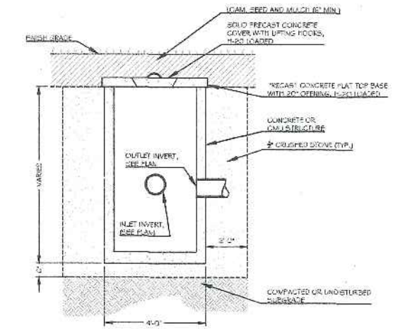
3 DRAINAGE MANHOLE C3.0 NOT TO SCALE
