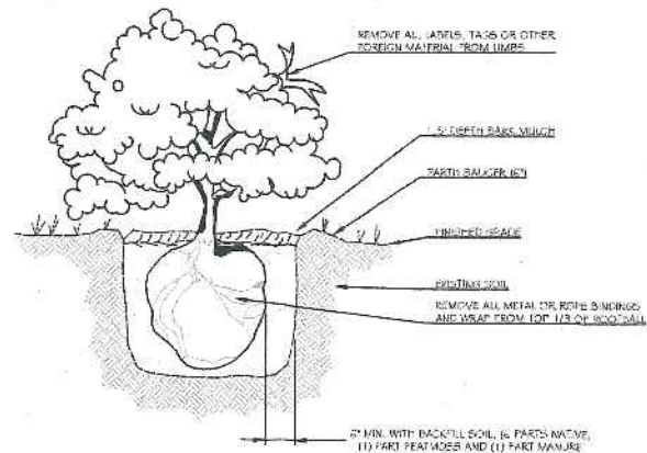
4 SHRUB PLANTING INSTALLATION C3.0 NOT TO SCALE
