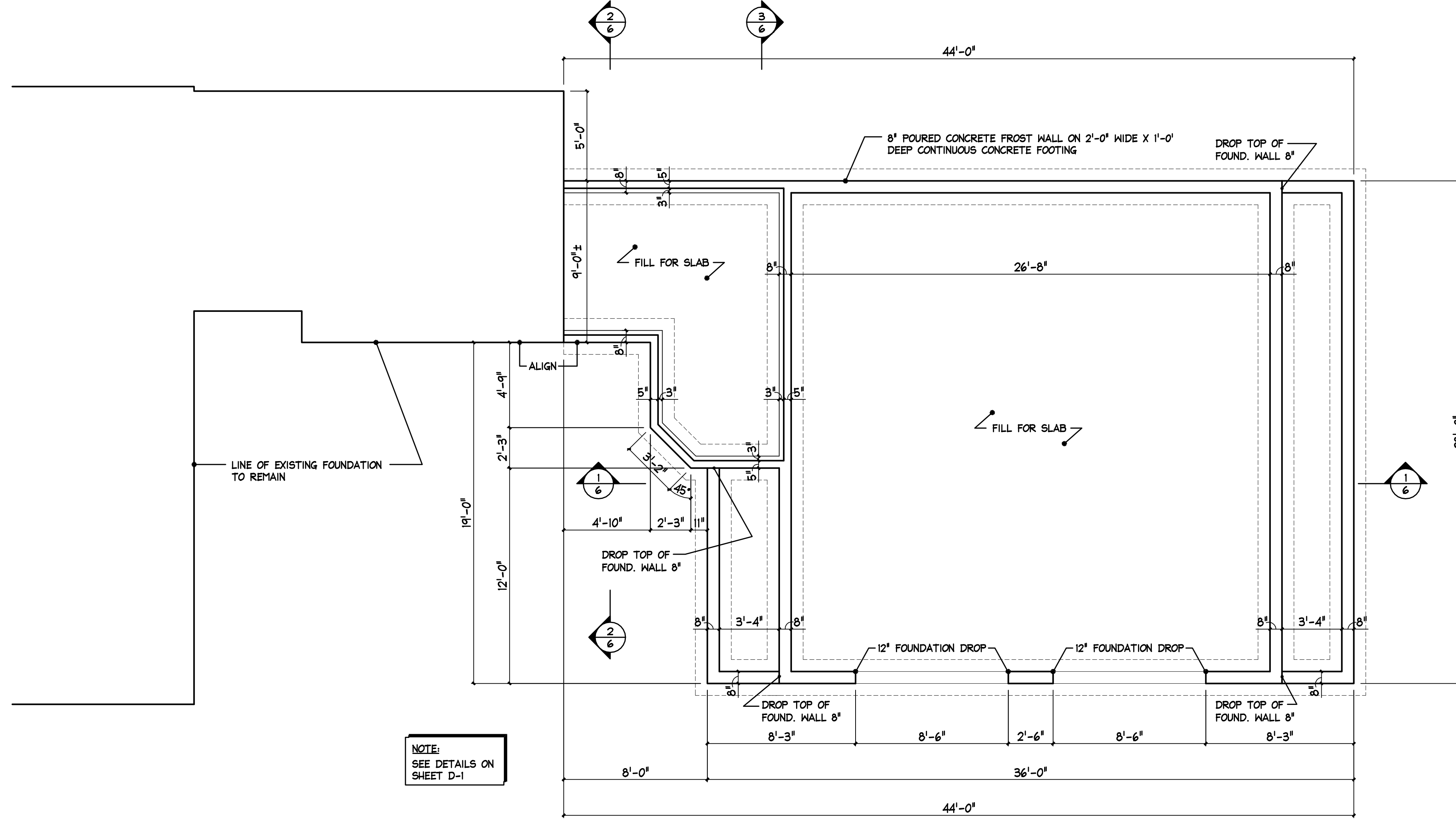
FOUNDATION PLAN 1/4" = 1'-0"
