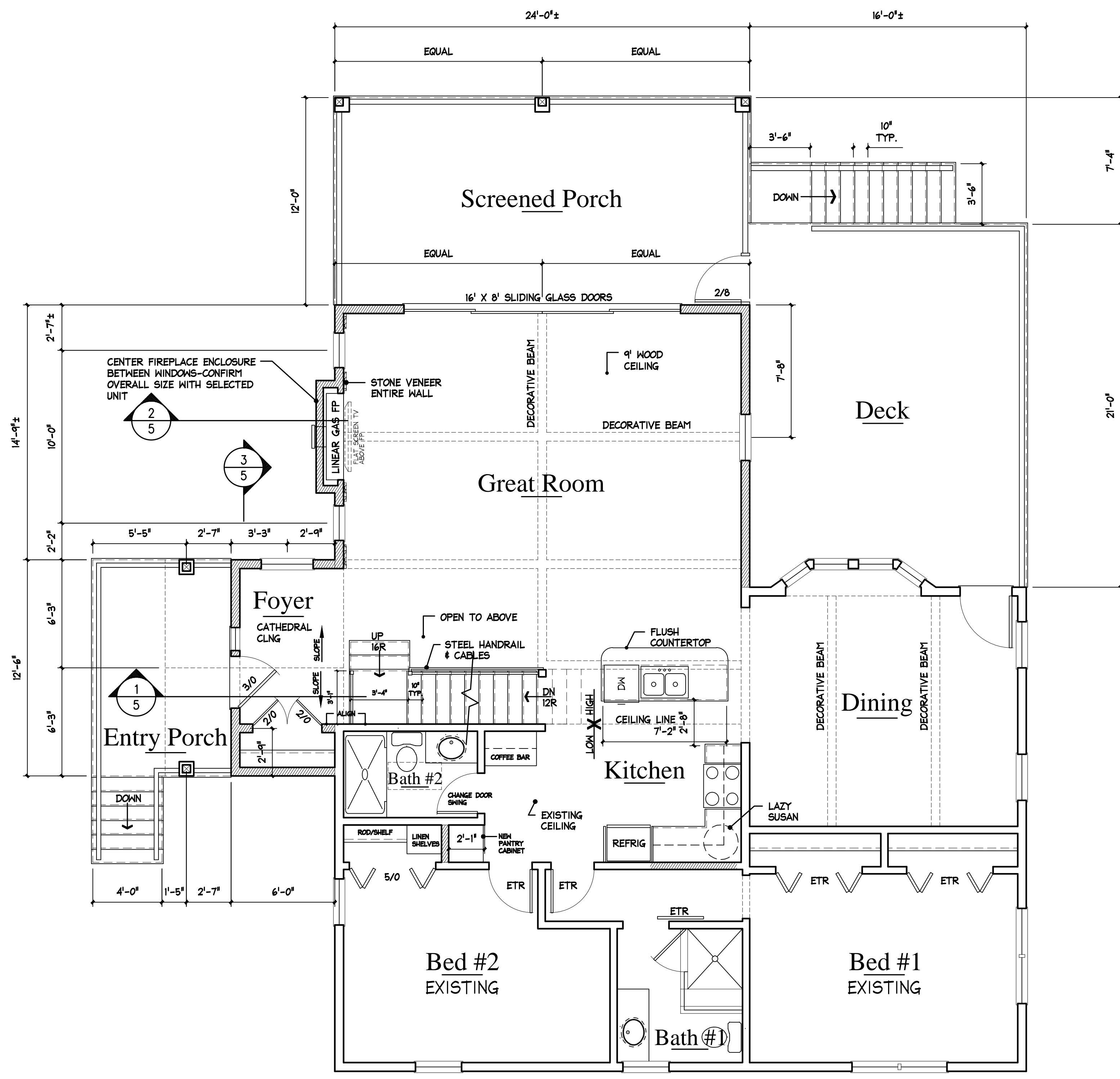
FIRST FLOOR PLAN 1/4" = 1'-0" ETR: EXISTING TO REMAIN
