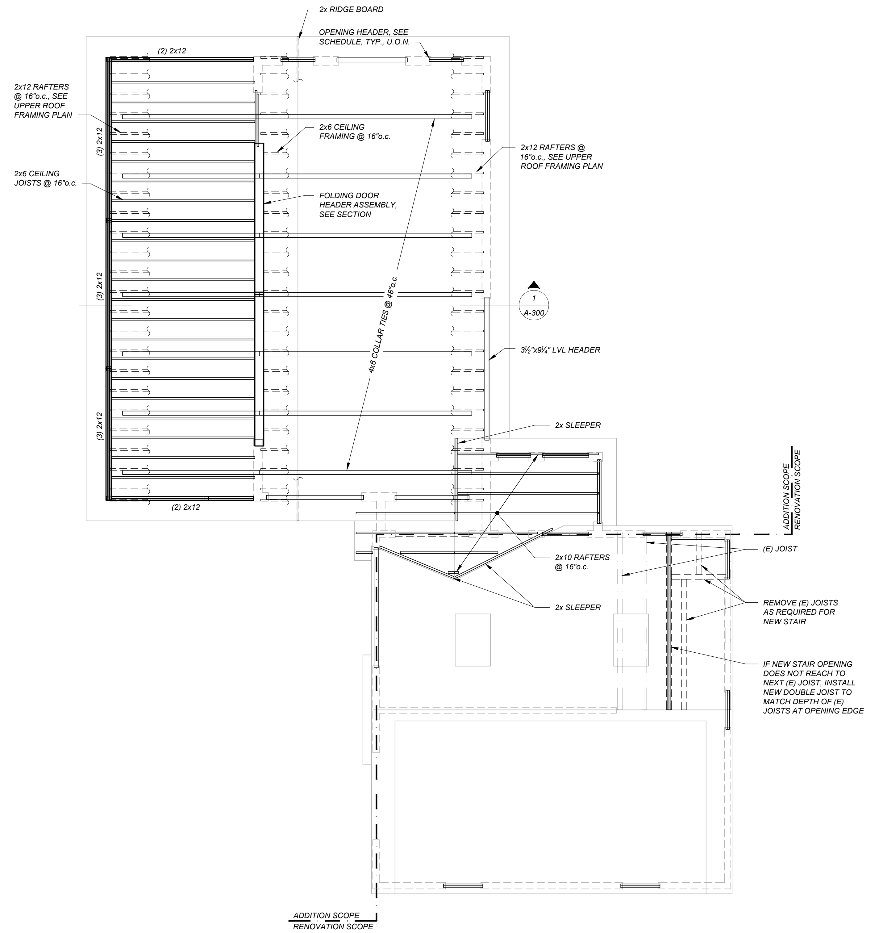
CEILING/ROOF FRAMING PLAN 1
