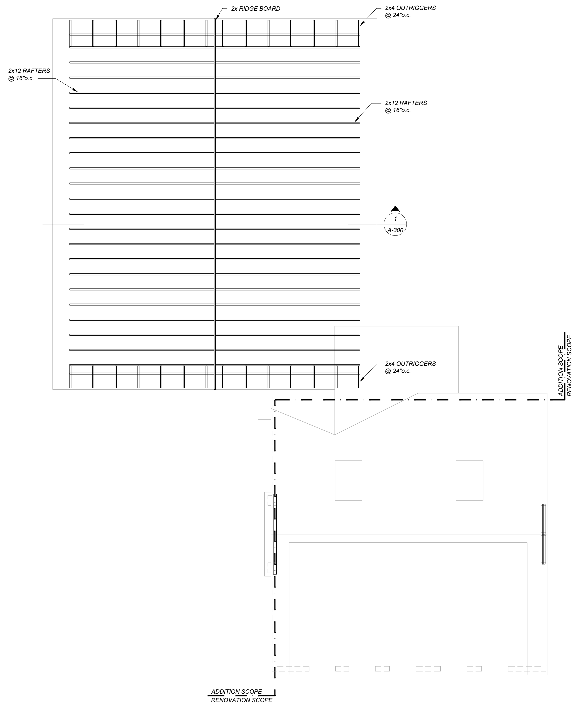
UPPER ROOF FRAMING PLAN 2
