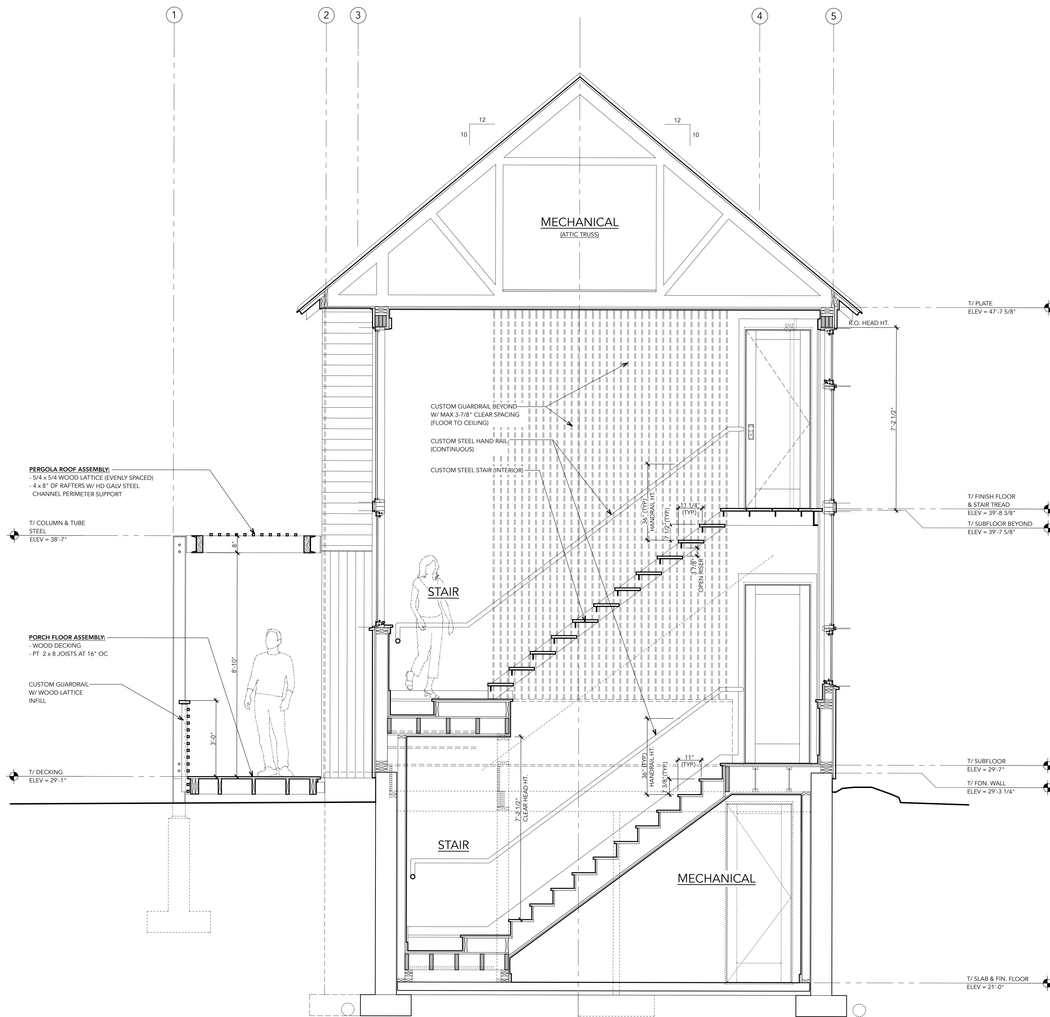
1 BUILDING SECTION (LOOKING EAST) SCALE: 1/2" = 1'-0"
