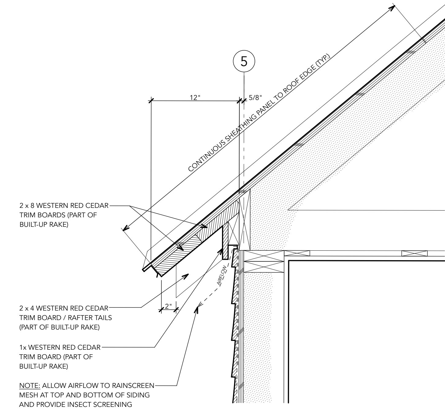
3 ROOF EAVE DETAIL (TYP.) SCALE: 1-1/2" = 1'-0"
