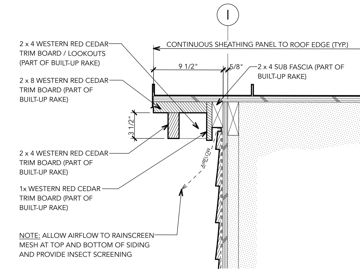
2 ROOF RAKE DETAIL (TYP.) SCALE: 1-1/2" = 1'-0"
