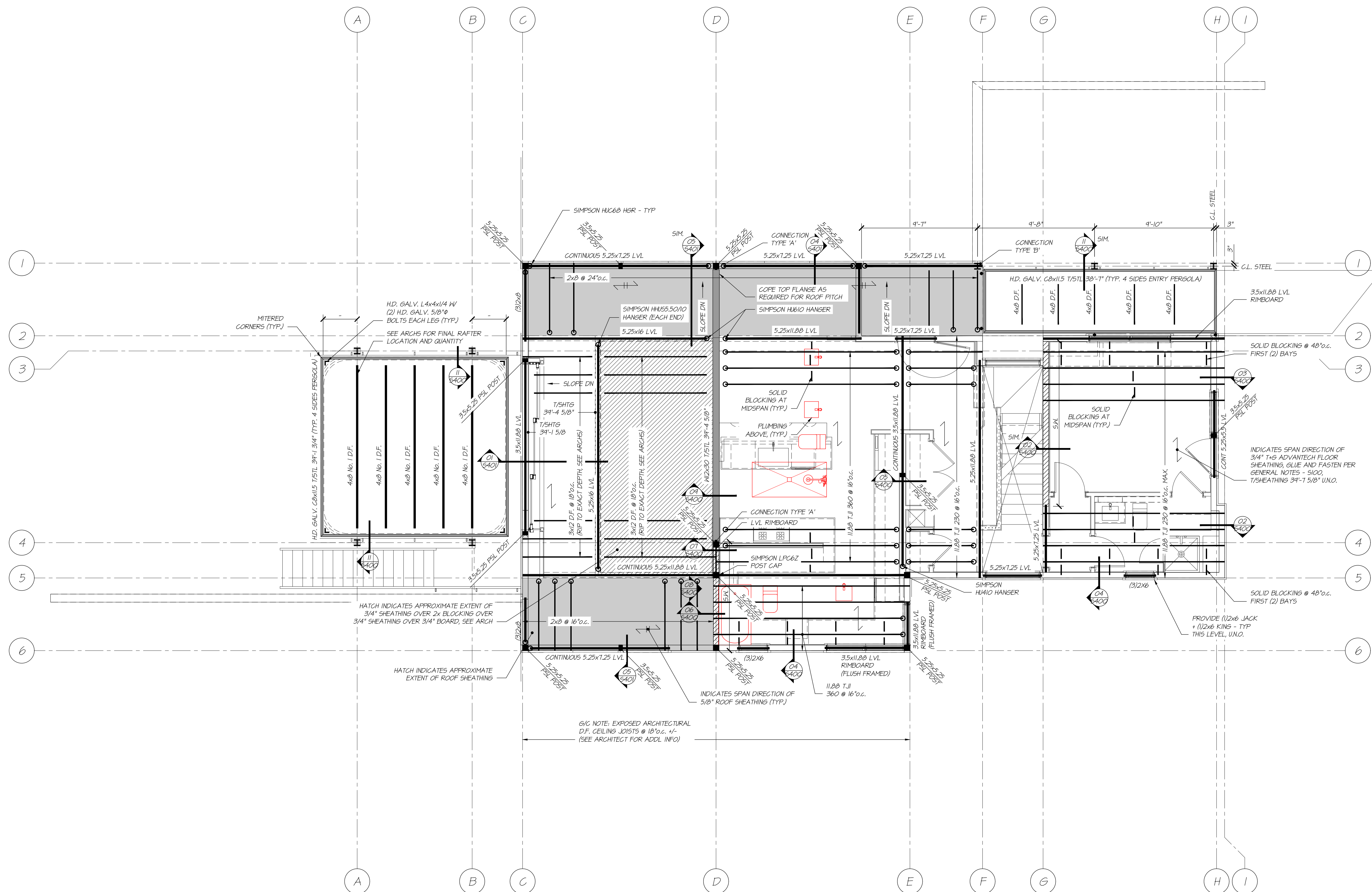
UPPER LEVEL FRAMING PLAN 1/4" = 1'-0"
