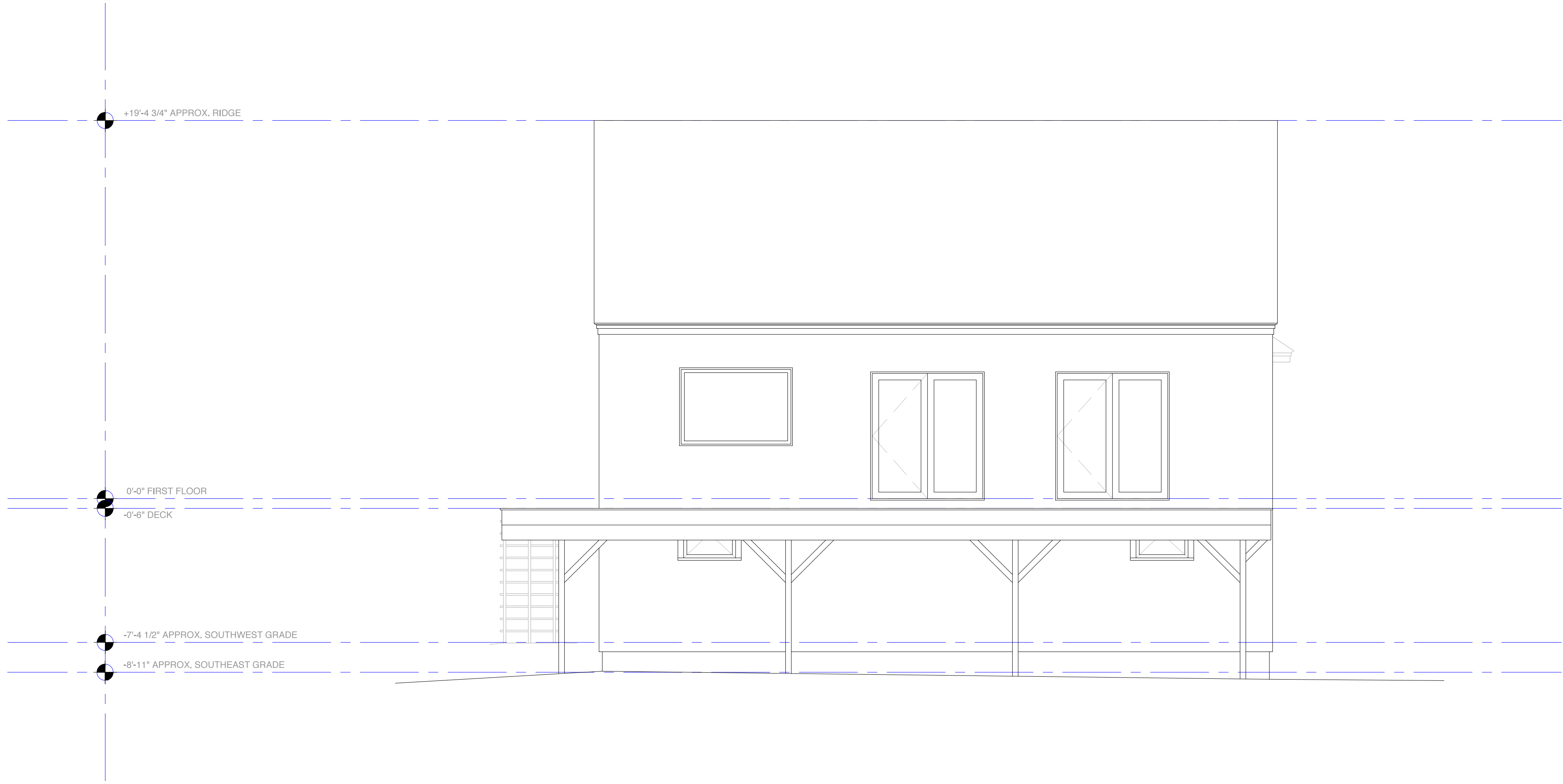
A Existing East Elevation 1/4" = 1'-0"
