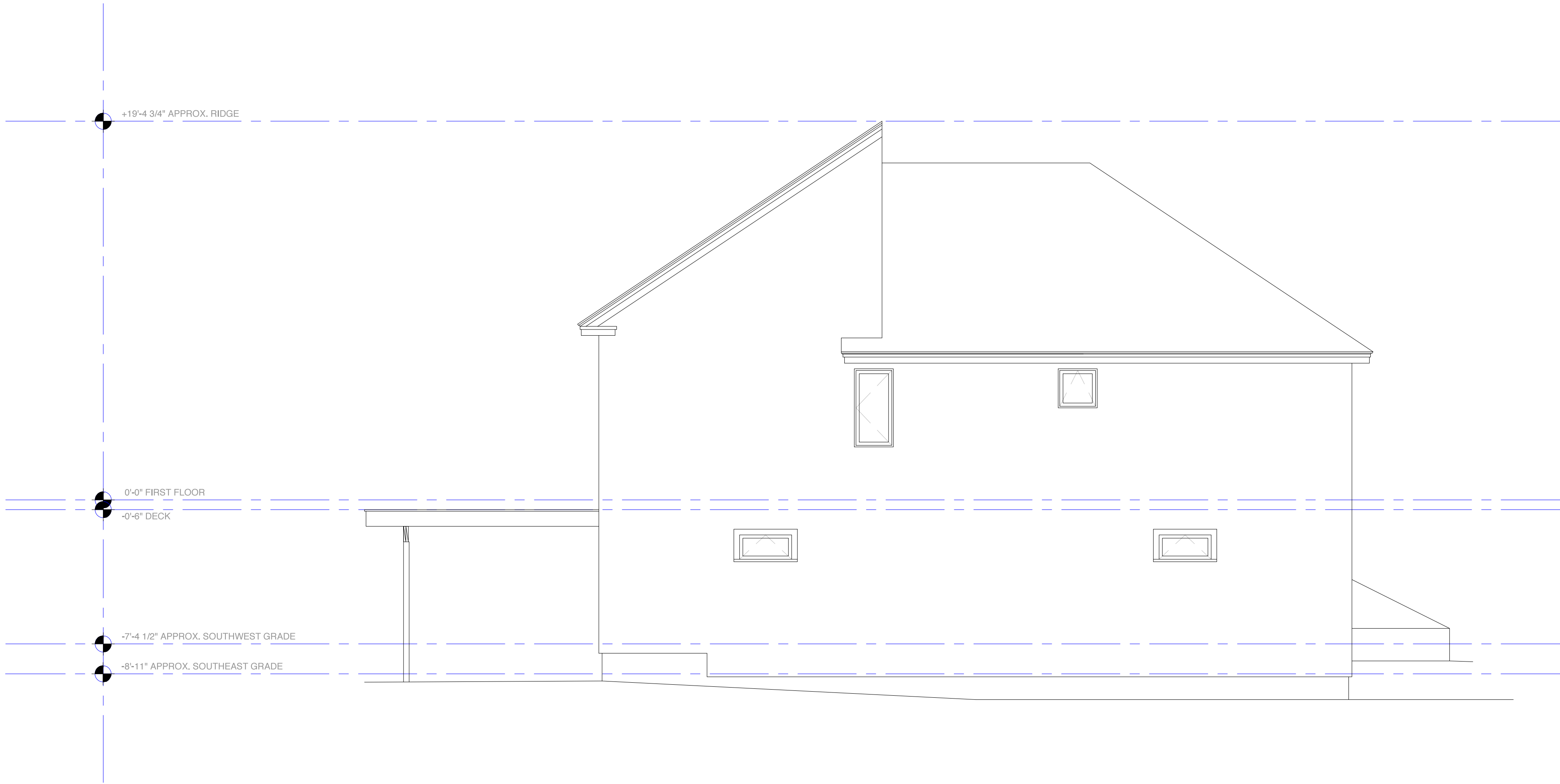
A Existing North Elevation 1/4" = 1'-0"
