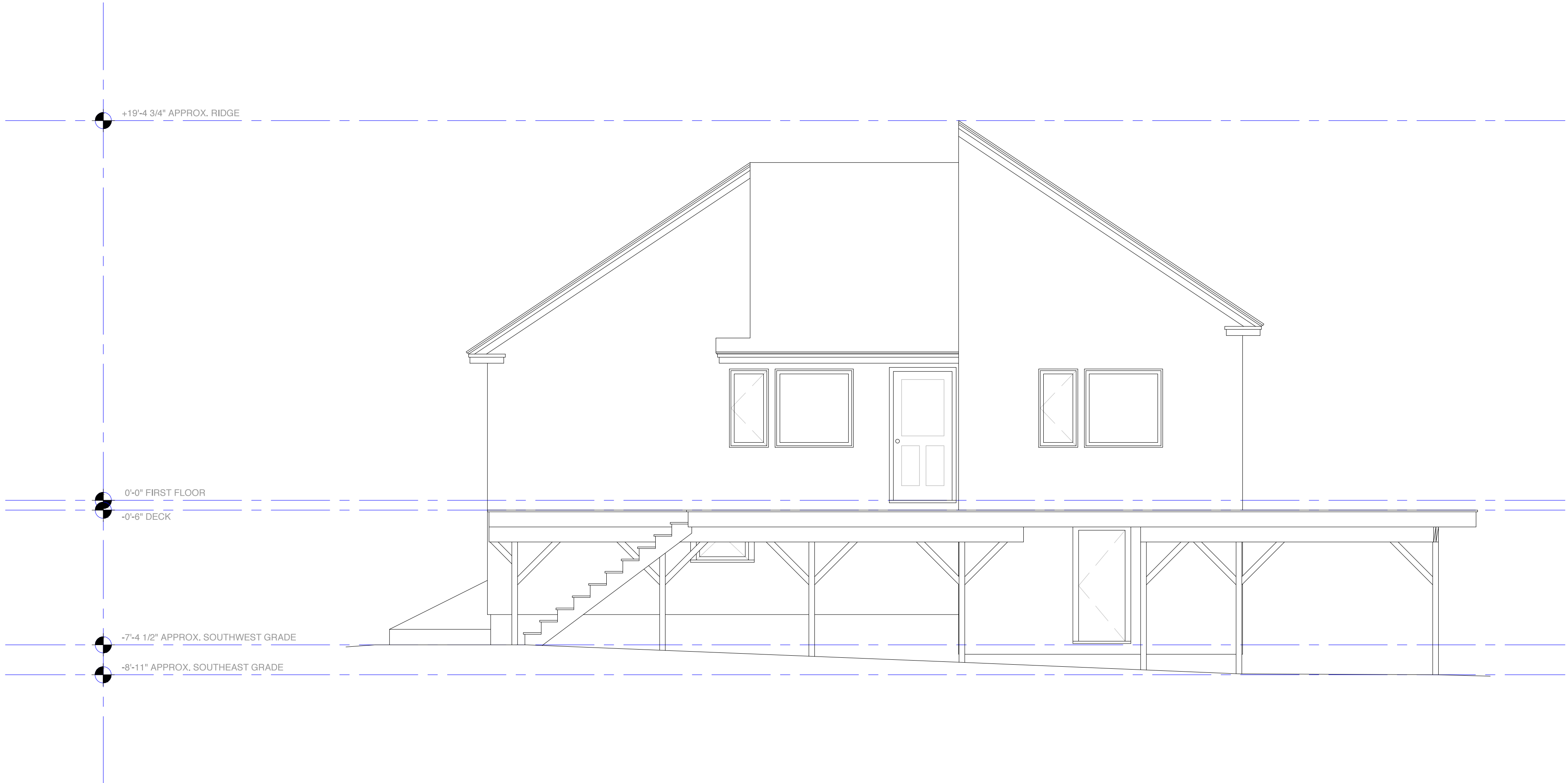
A Existing South Elevation 1/4" = 1'-0"
