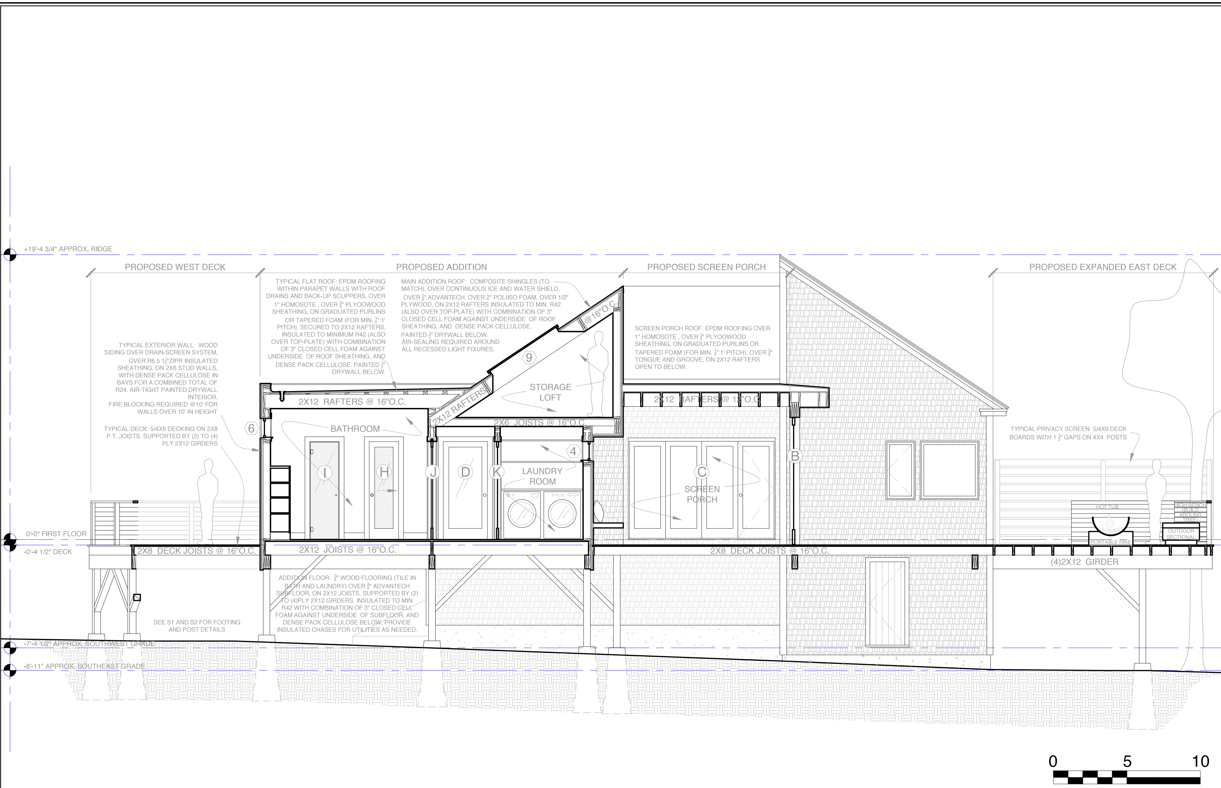
A Proposed Cross Section
