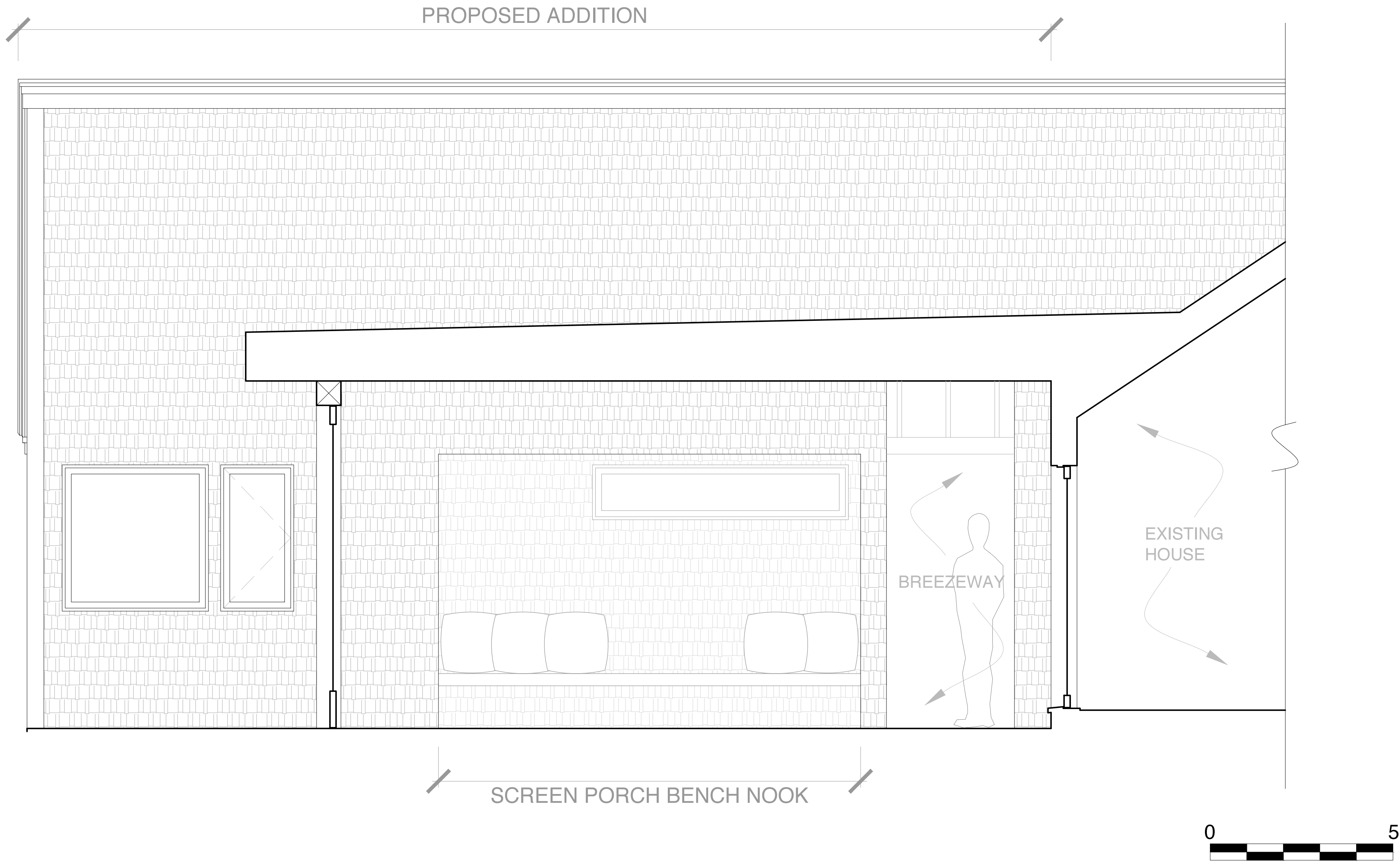
A Proposed Covered Porch West Elevation
