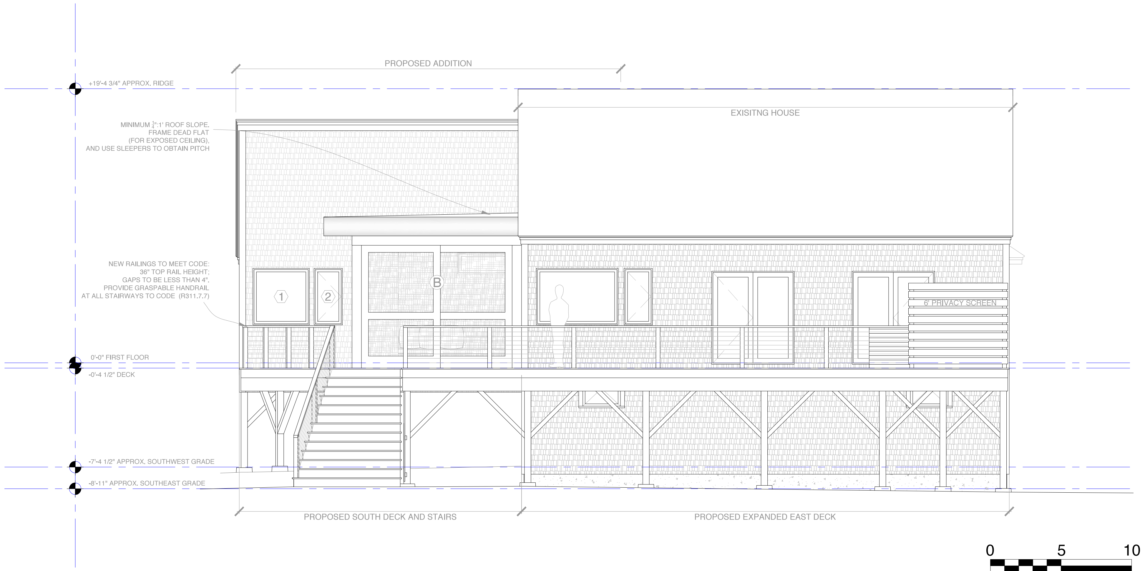
A Proposed East Elevation
