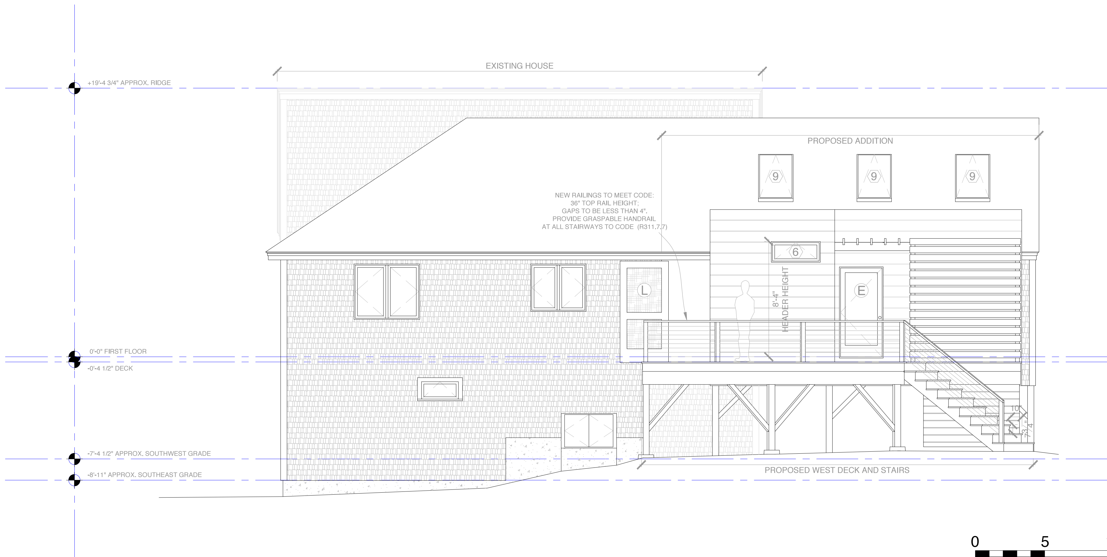
A Proposed West Elevation
