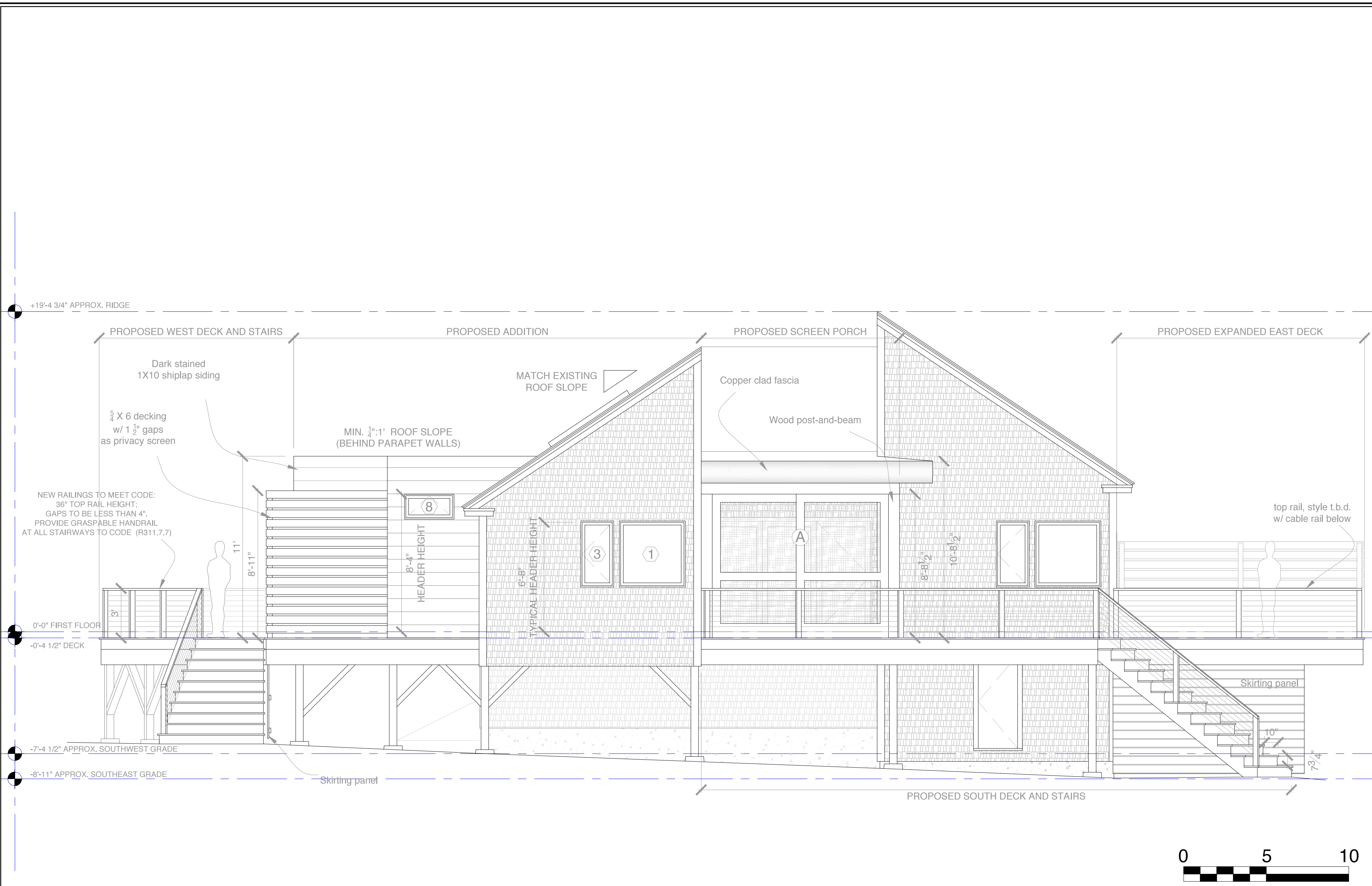
A Proposed South Elevation
