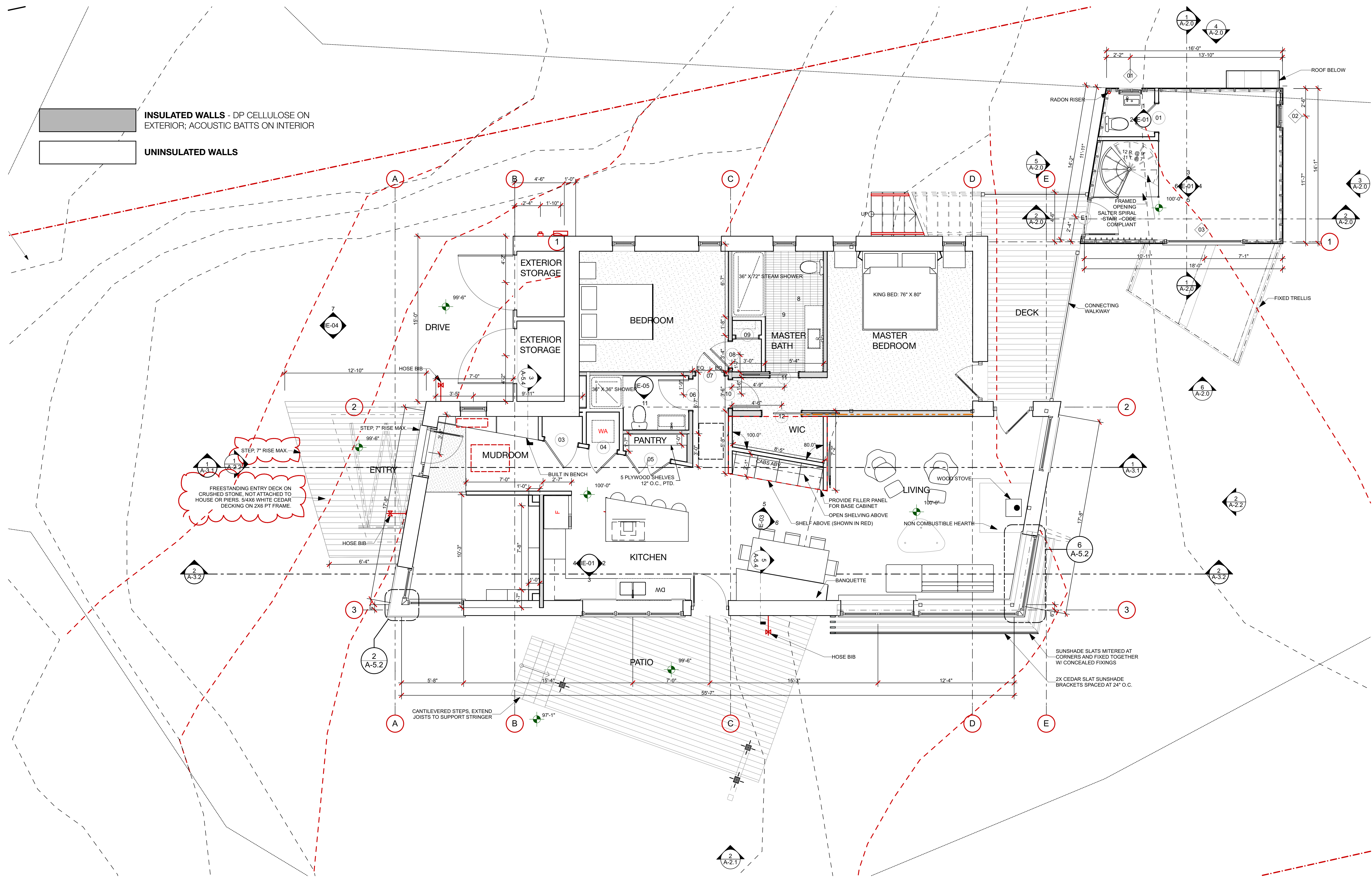
1st FLOOR SCALE: 1/4" = 1'-0"
