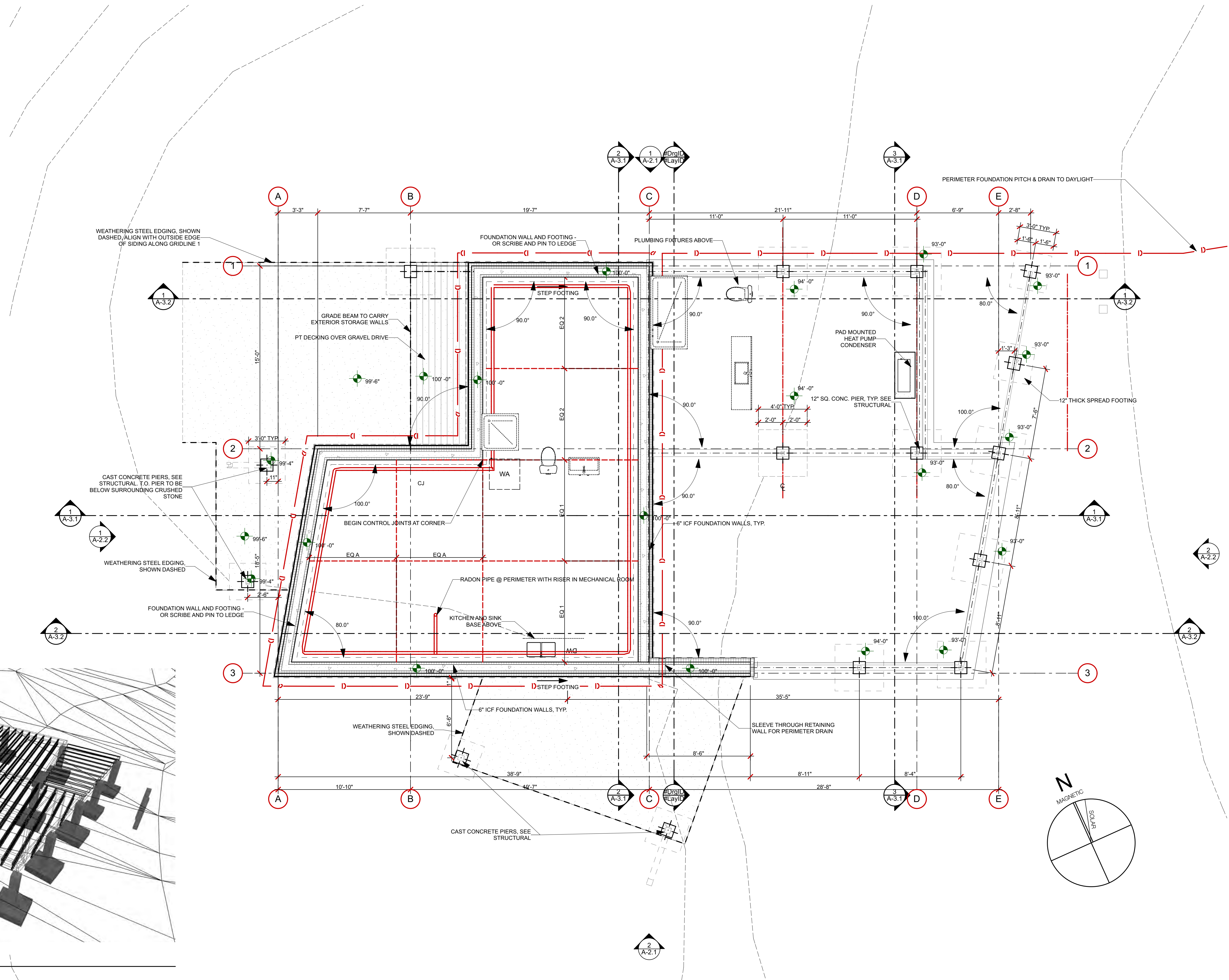
1 FOUNDATION SCALE: 1/4" = 1'-0"
