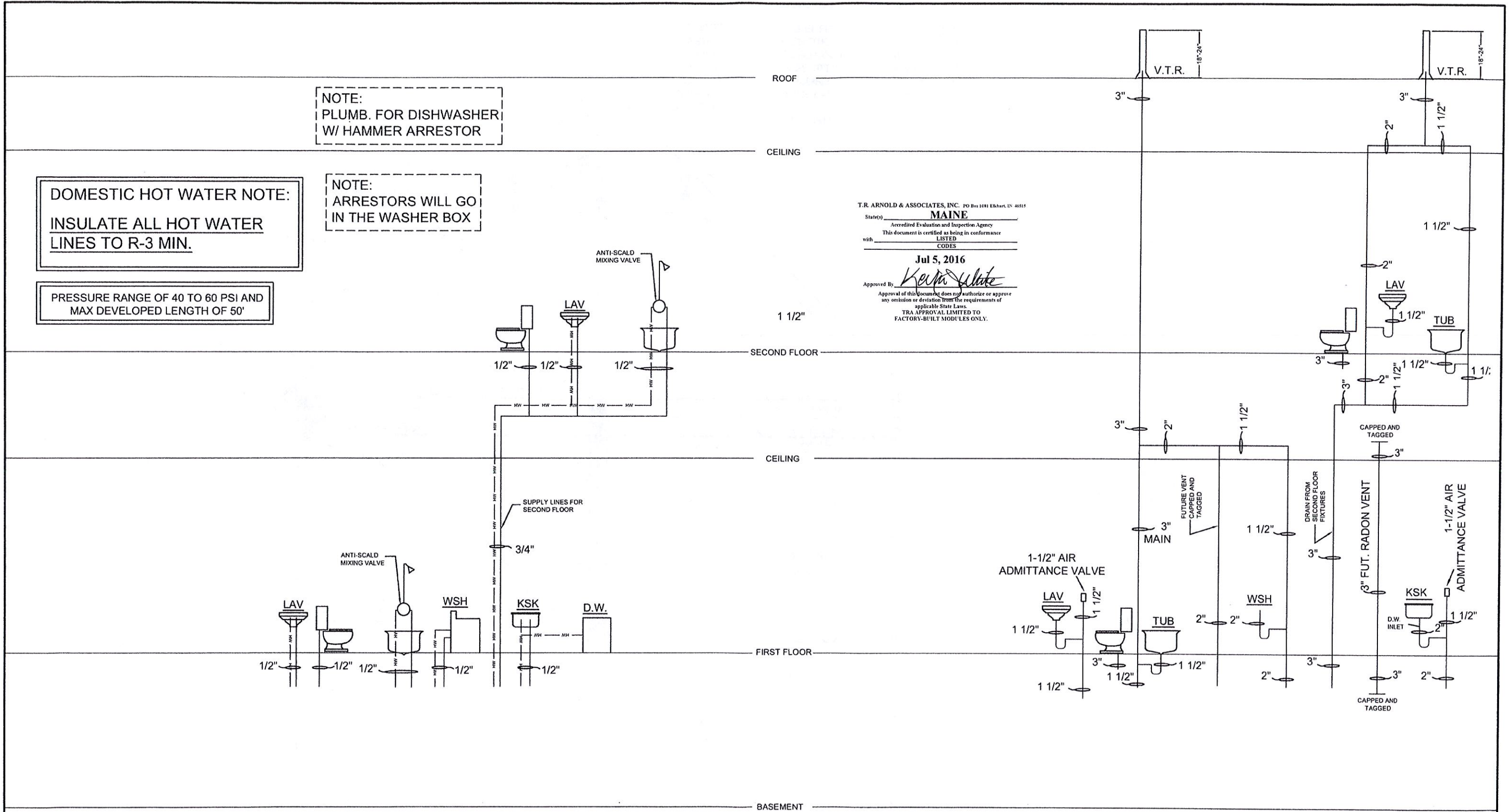
TYPICAL SUPPLY. SCHEMATIC - NOT TO SCALE
