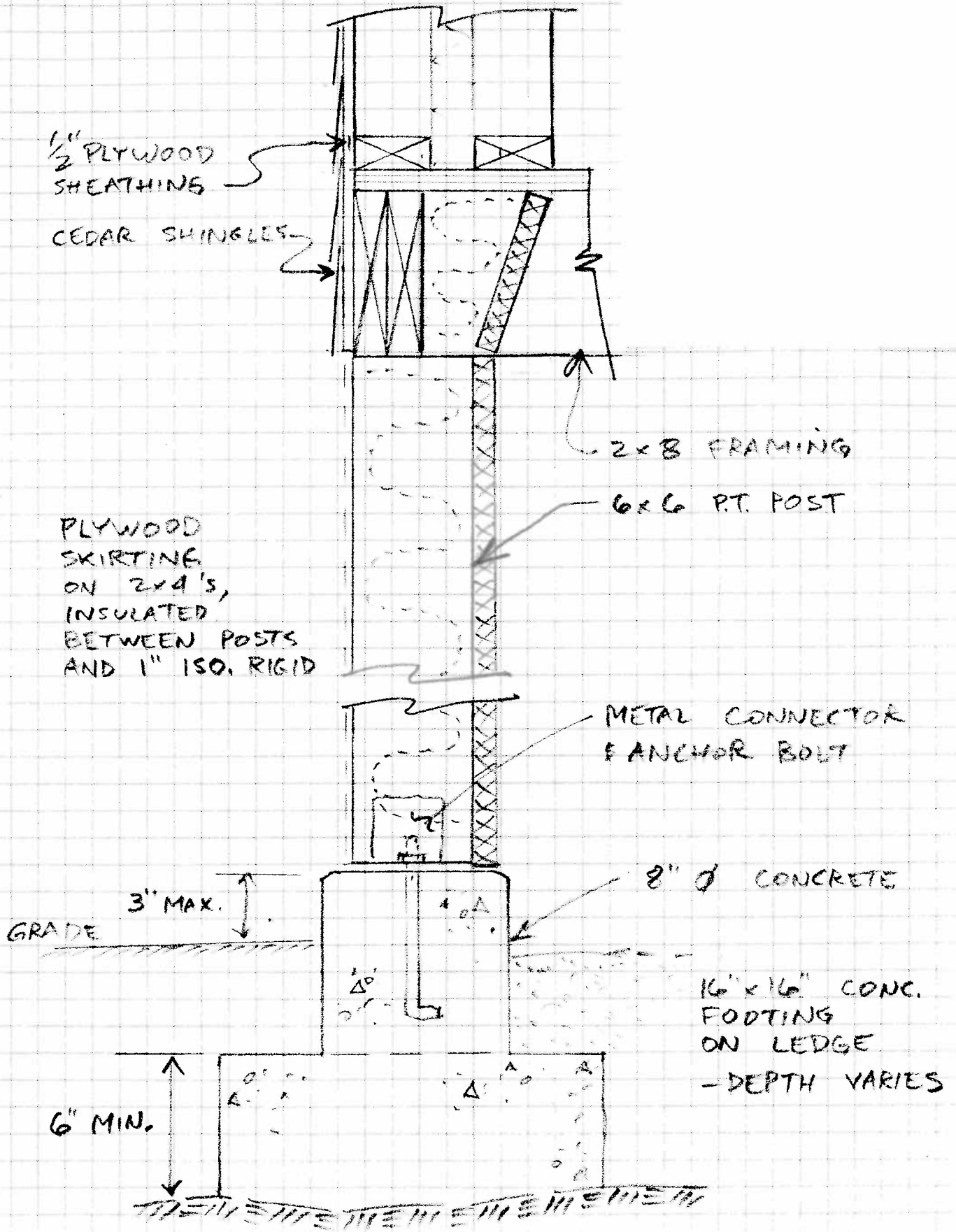
A-10: POSTS AT NORTH WALL (SECTION)
