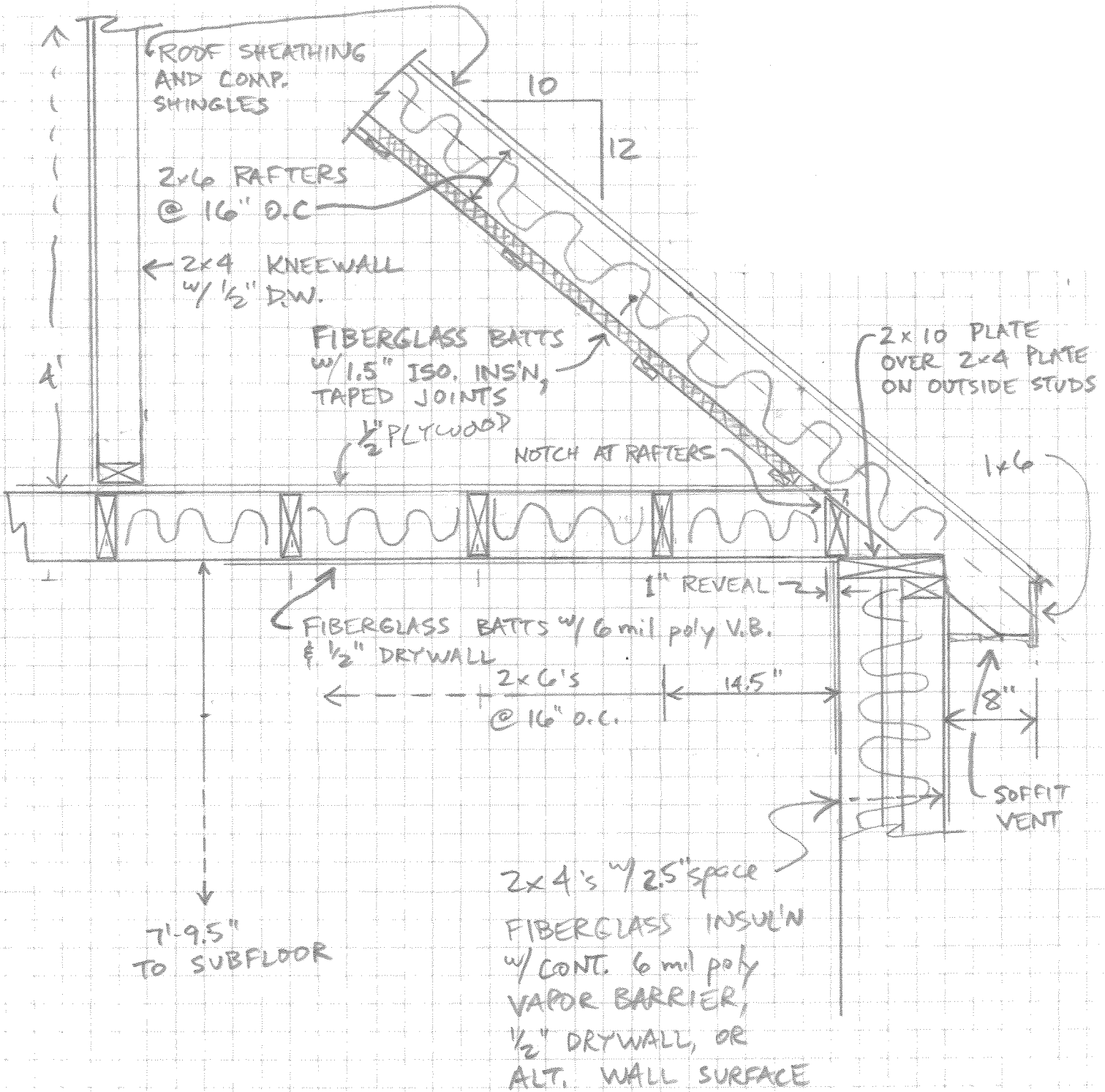
A-9: FRAMING SECTION (EAST-WEST)
