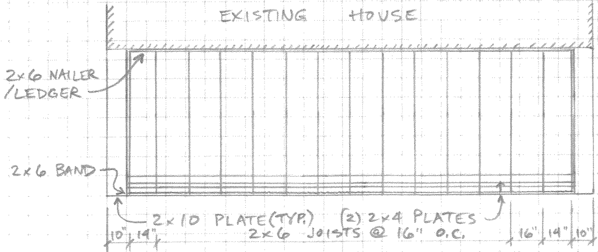
CEILING FRAMING PLAN
