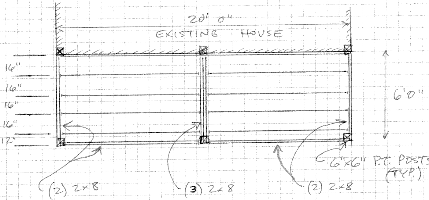
FRAMING A-7: FIRST FLOOR DECK ^ PLAN
