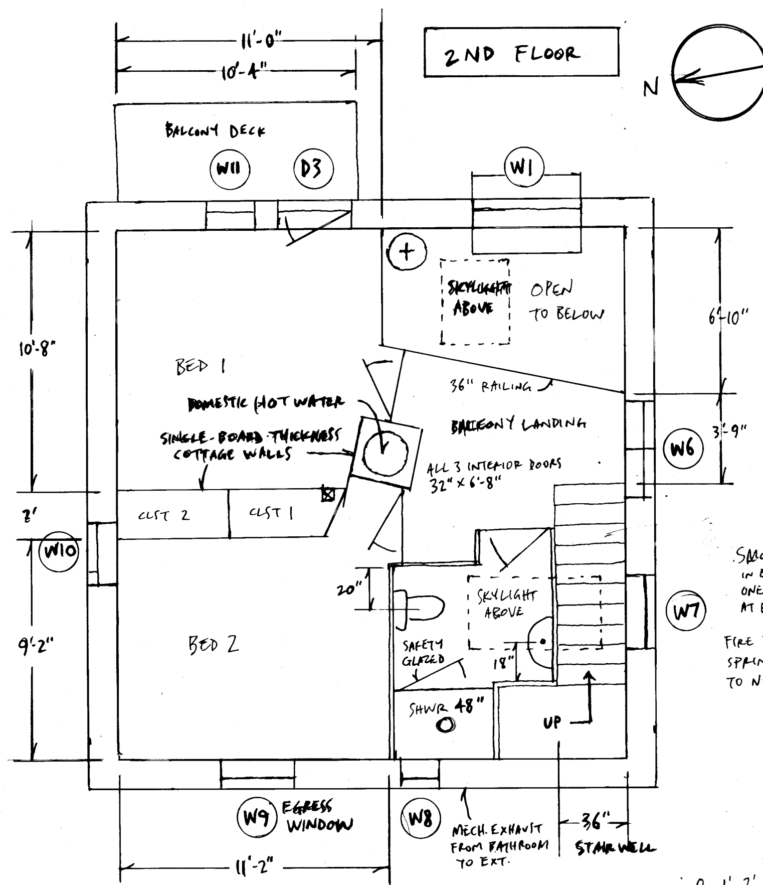
11.16.16 SPACE FLOOR PLAN - V.4-1'
