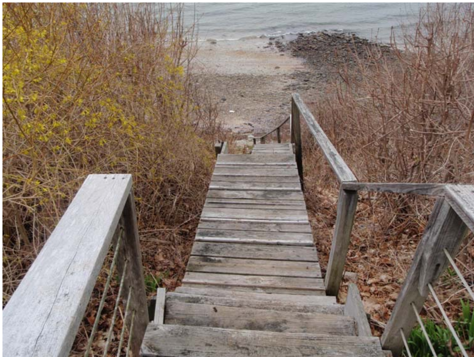
View of existing stair from lawn. Vegetation clearing required 2 ft either side of stair for new construction.
