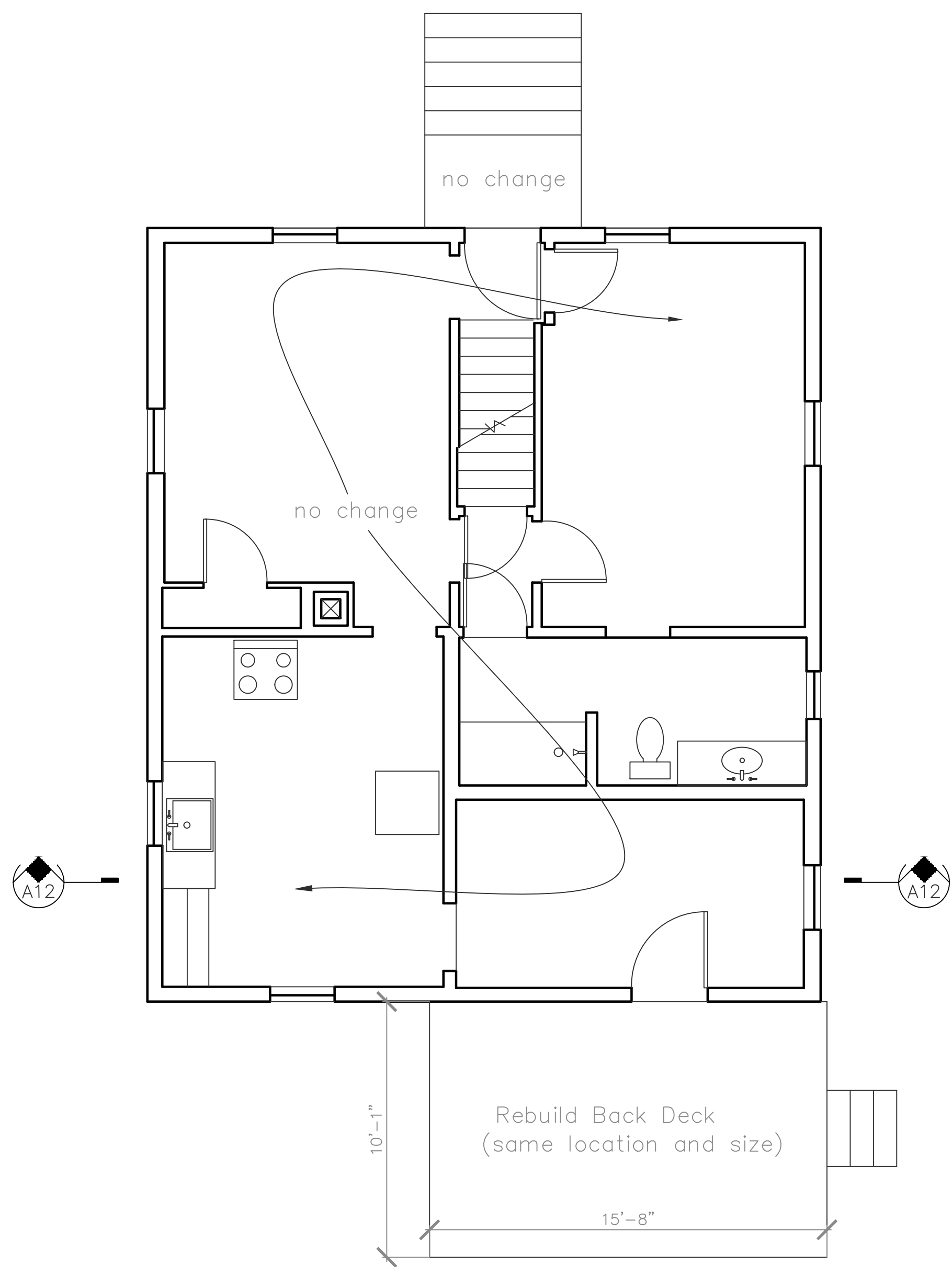
A Proposed First Floor, 1/4" = 1'-0"
