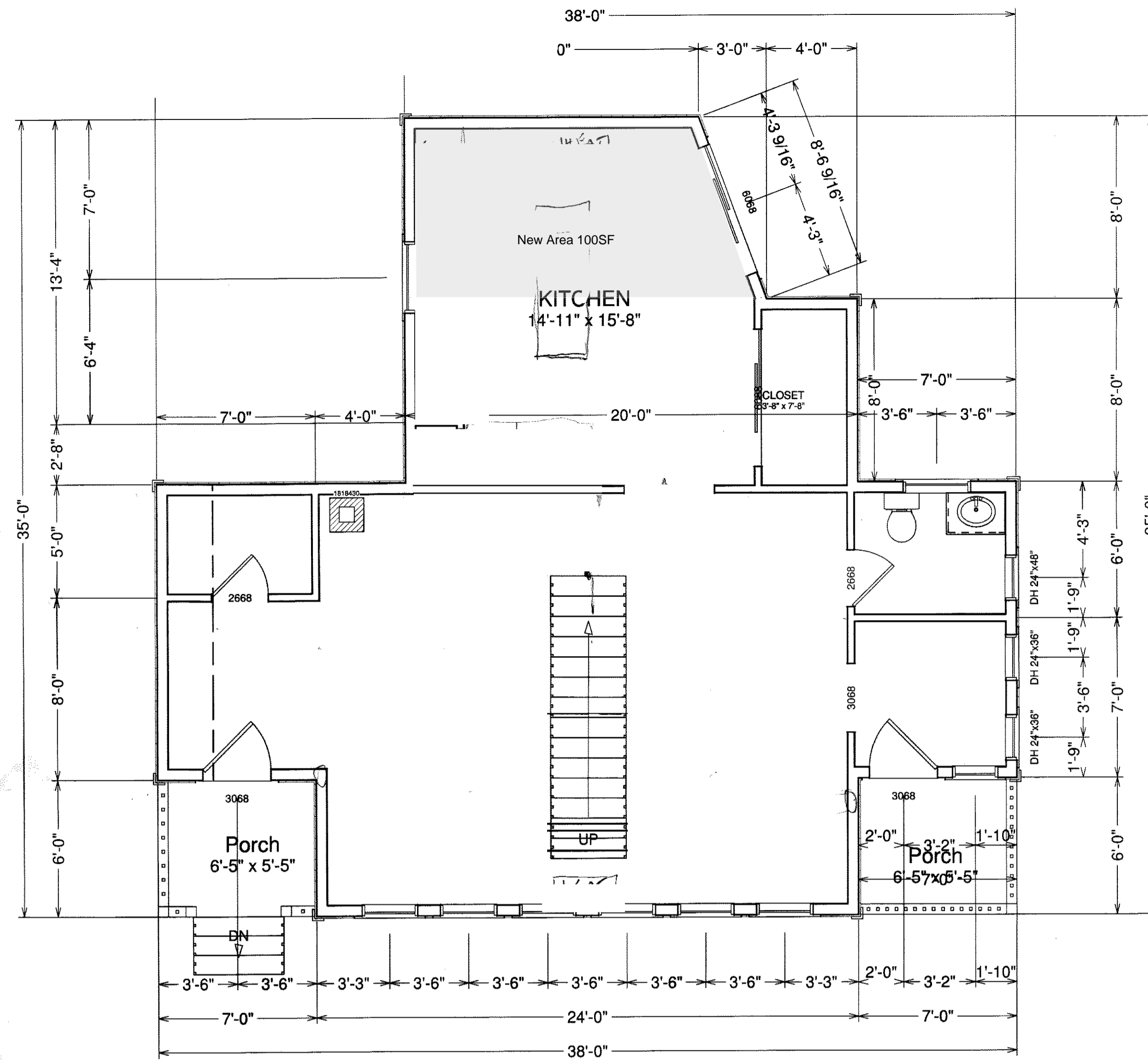
FIRST FLOOR Multiple Ceiling Hgts 915 sq ft Living Area
