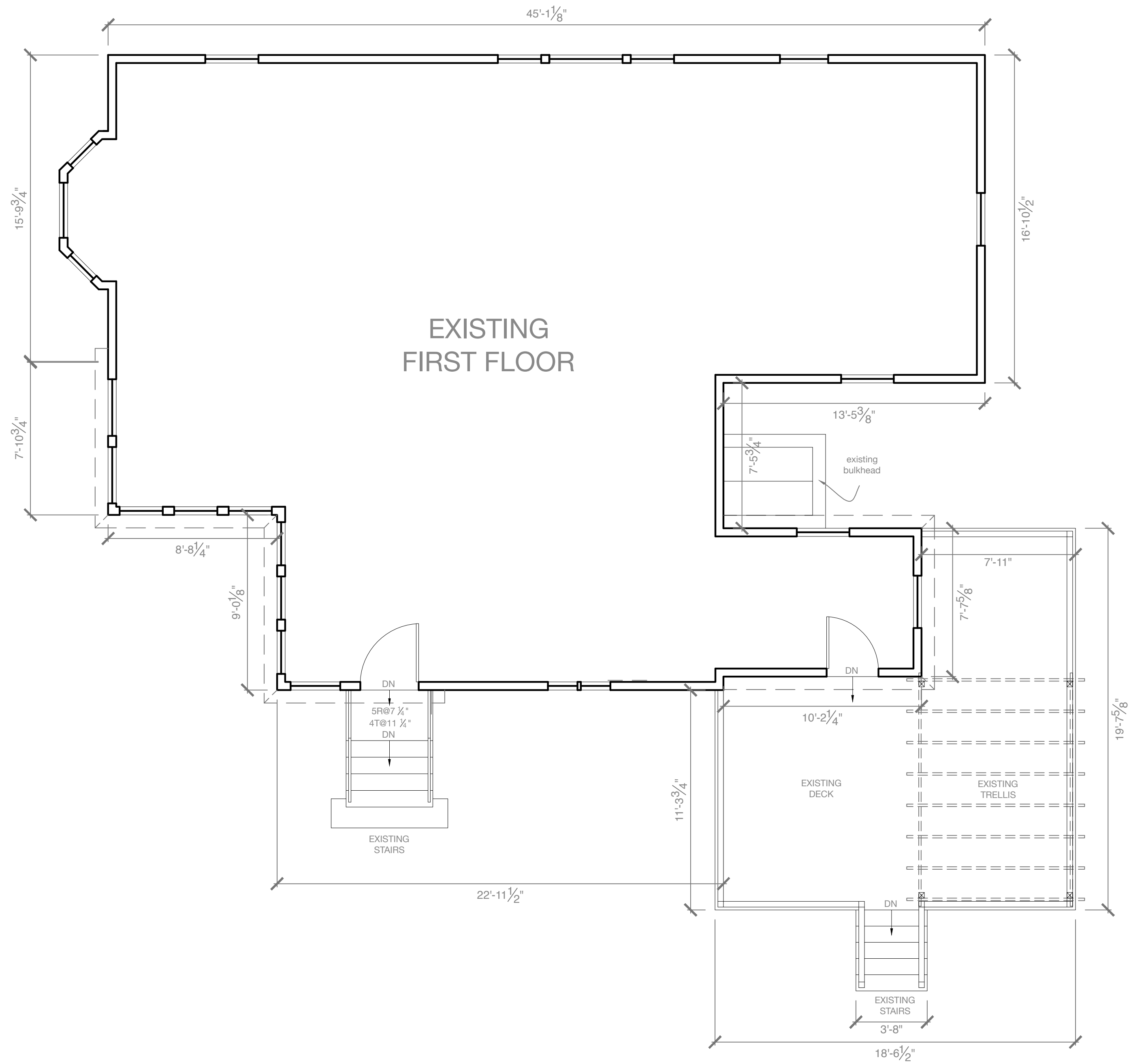
A Existing First Floor Plan
