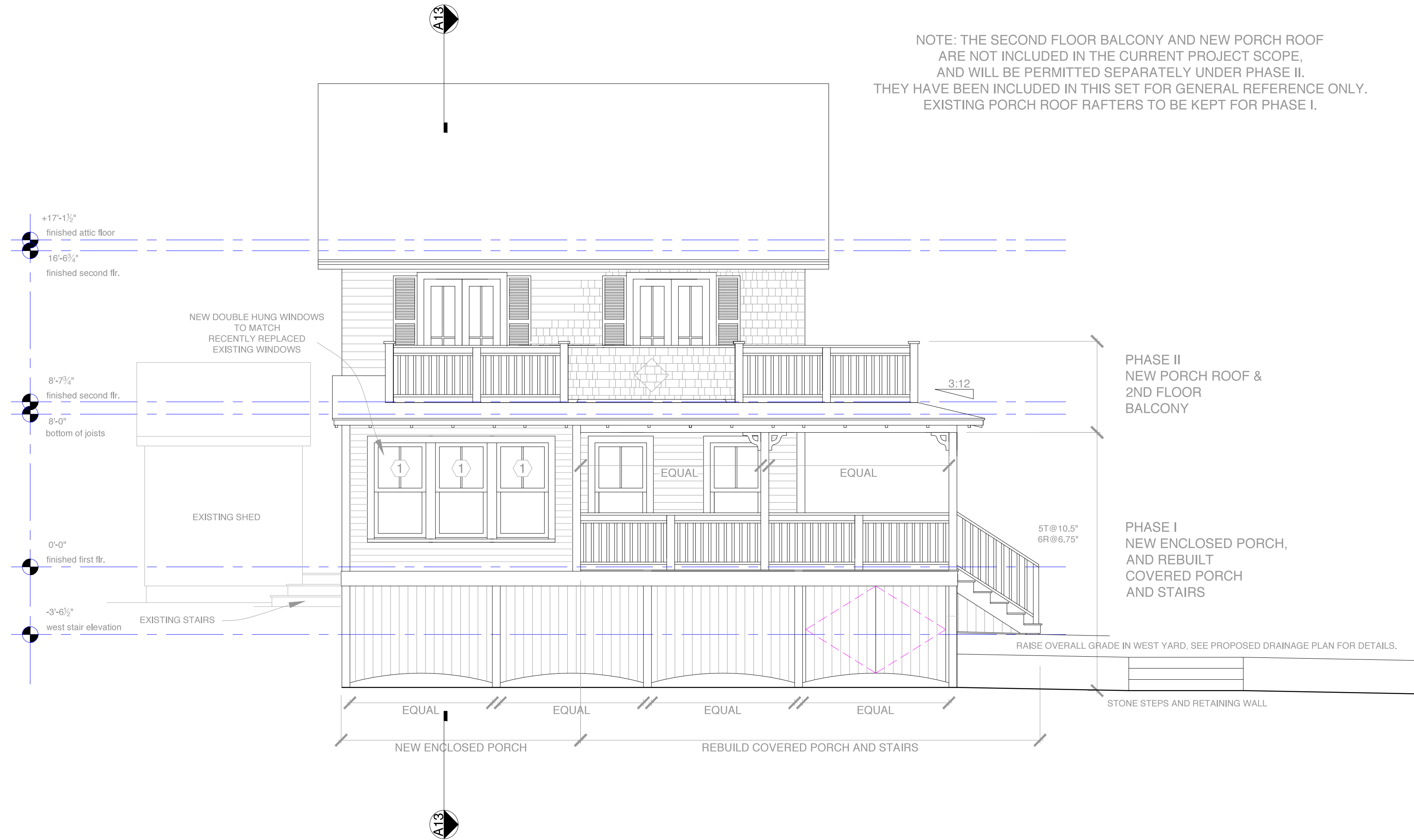
A Proposed North Elevation
