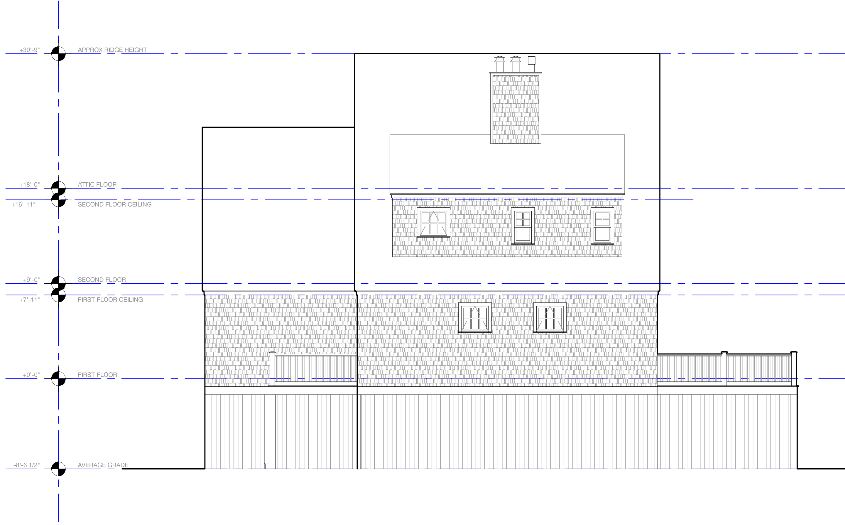
A Existing East Elevation
