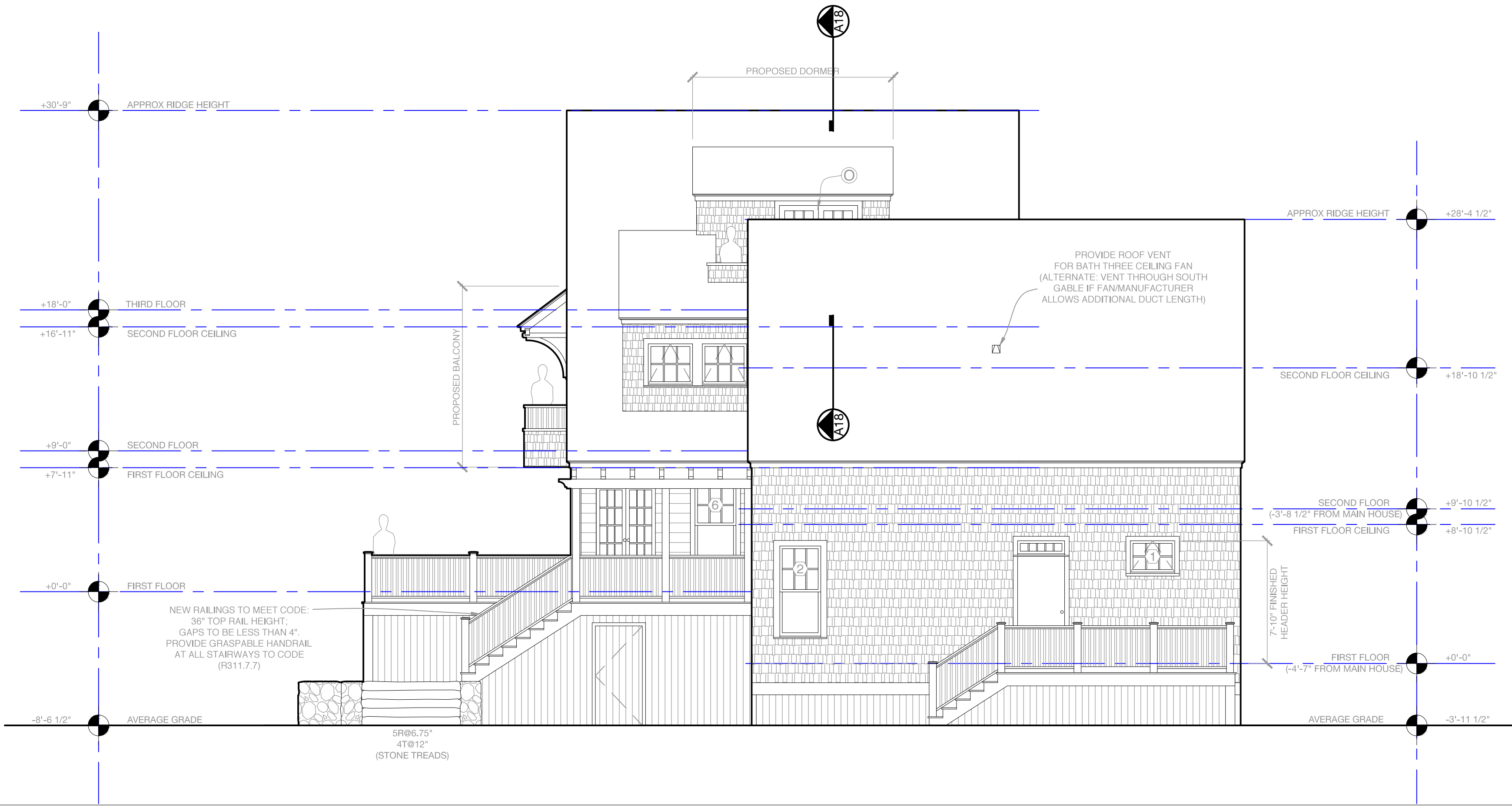
A Proposed West Elevation
