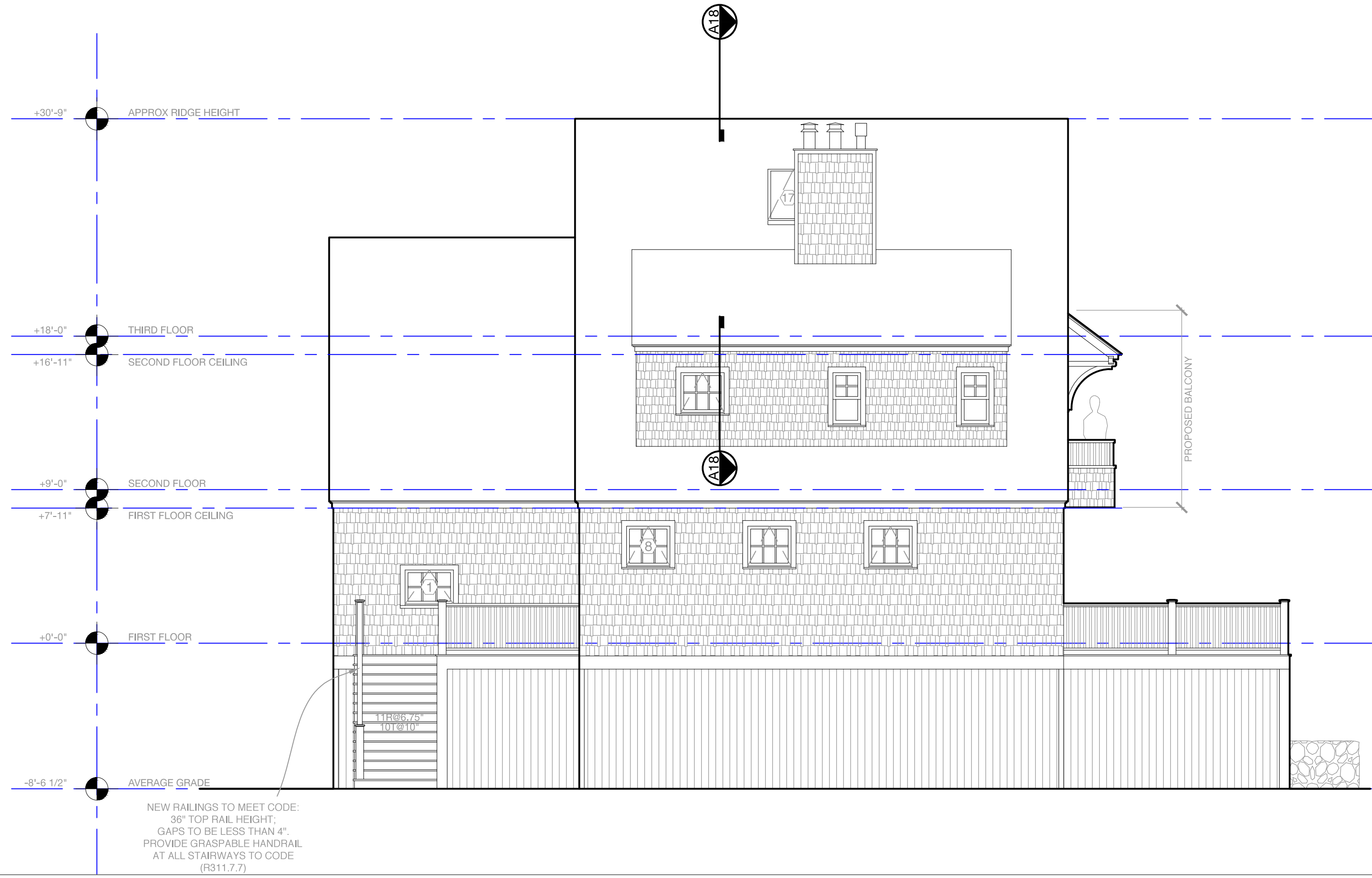
A Proposed East Elevation
