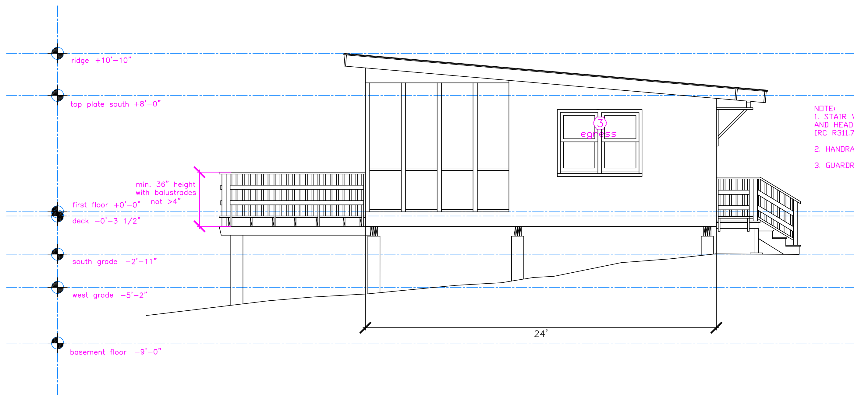
A Proposed West Elevation 1/4" = 1'-0"
