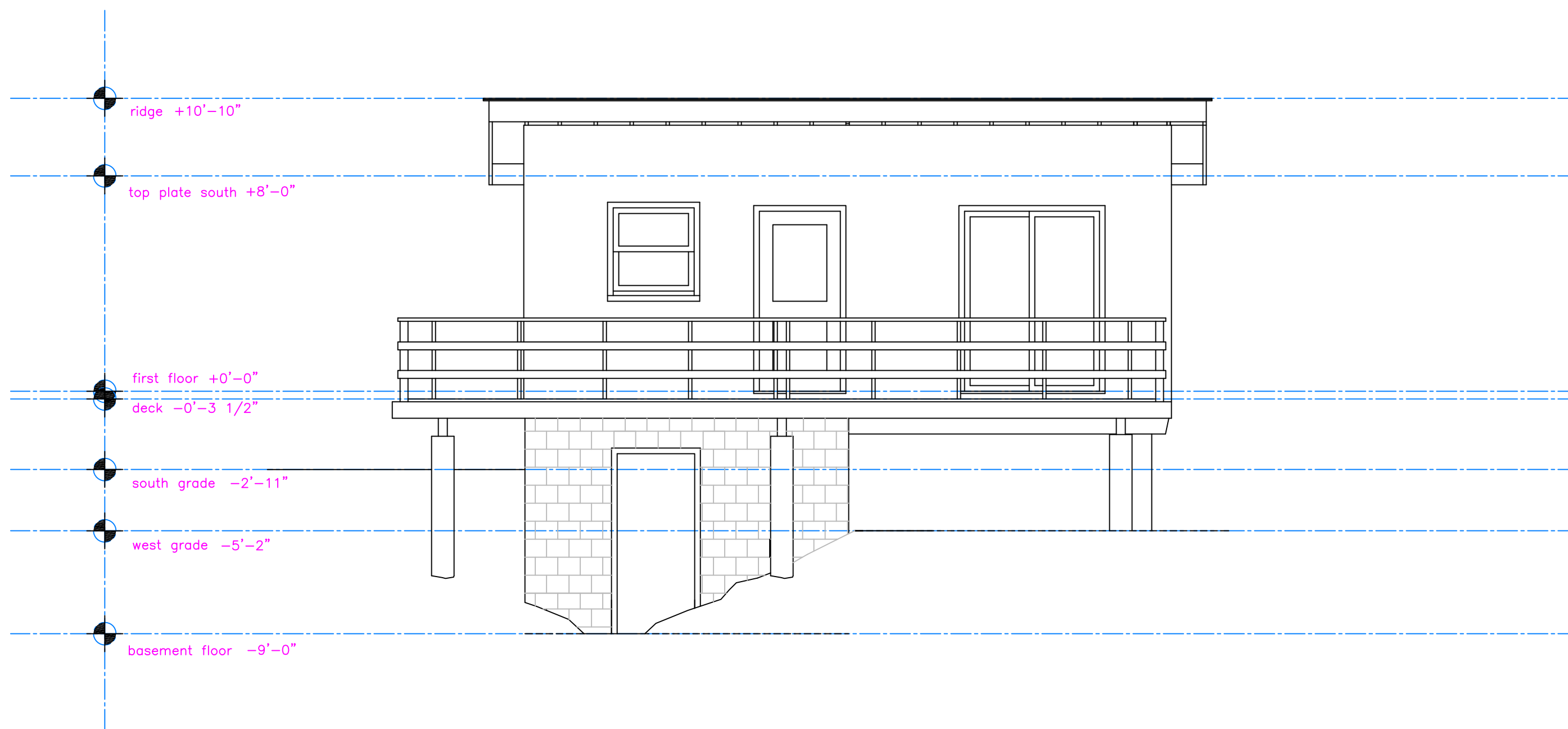
A Existing North Elevation 1/4" = 1'-0"
