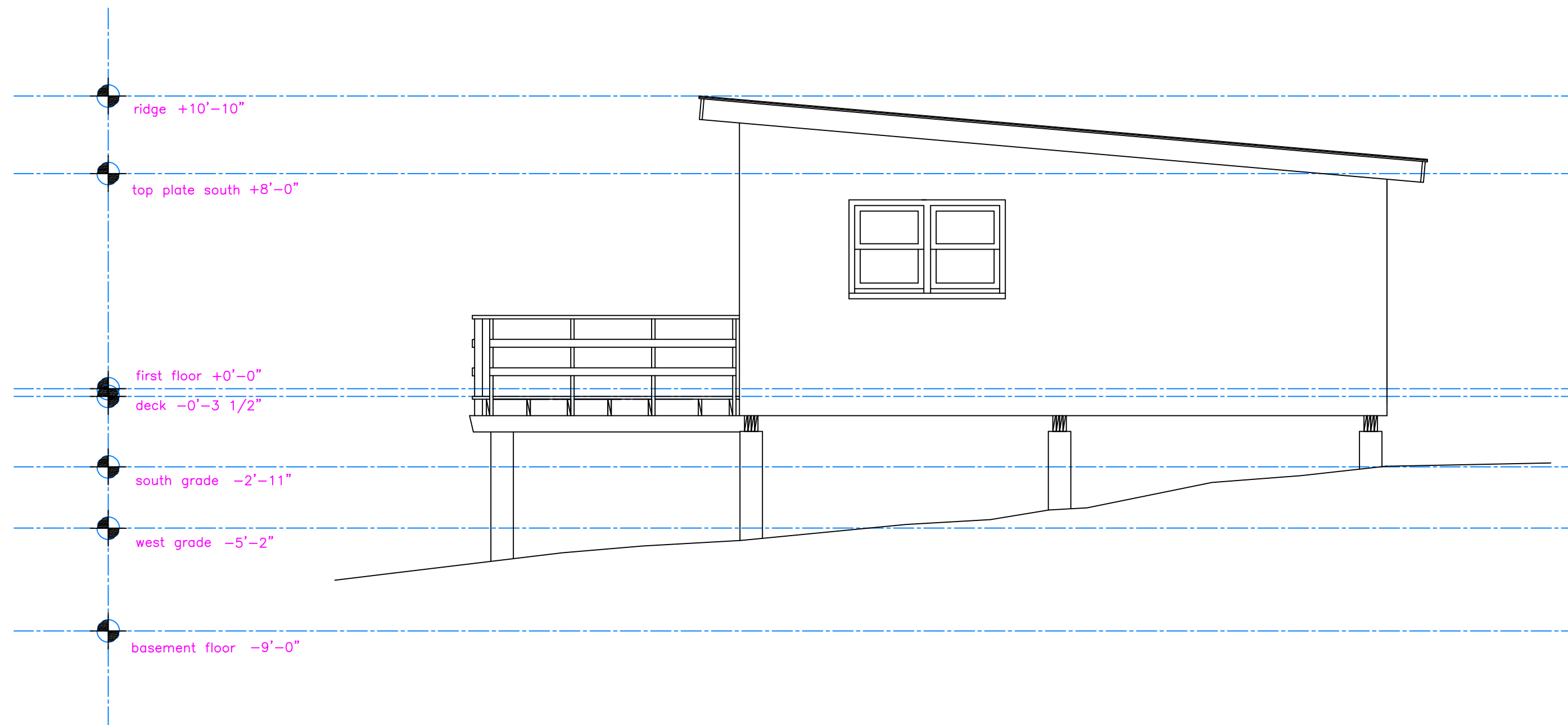
Ⓐ Existing West Elevation 1/4" = 1'-0"
