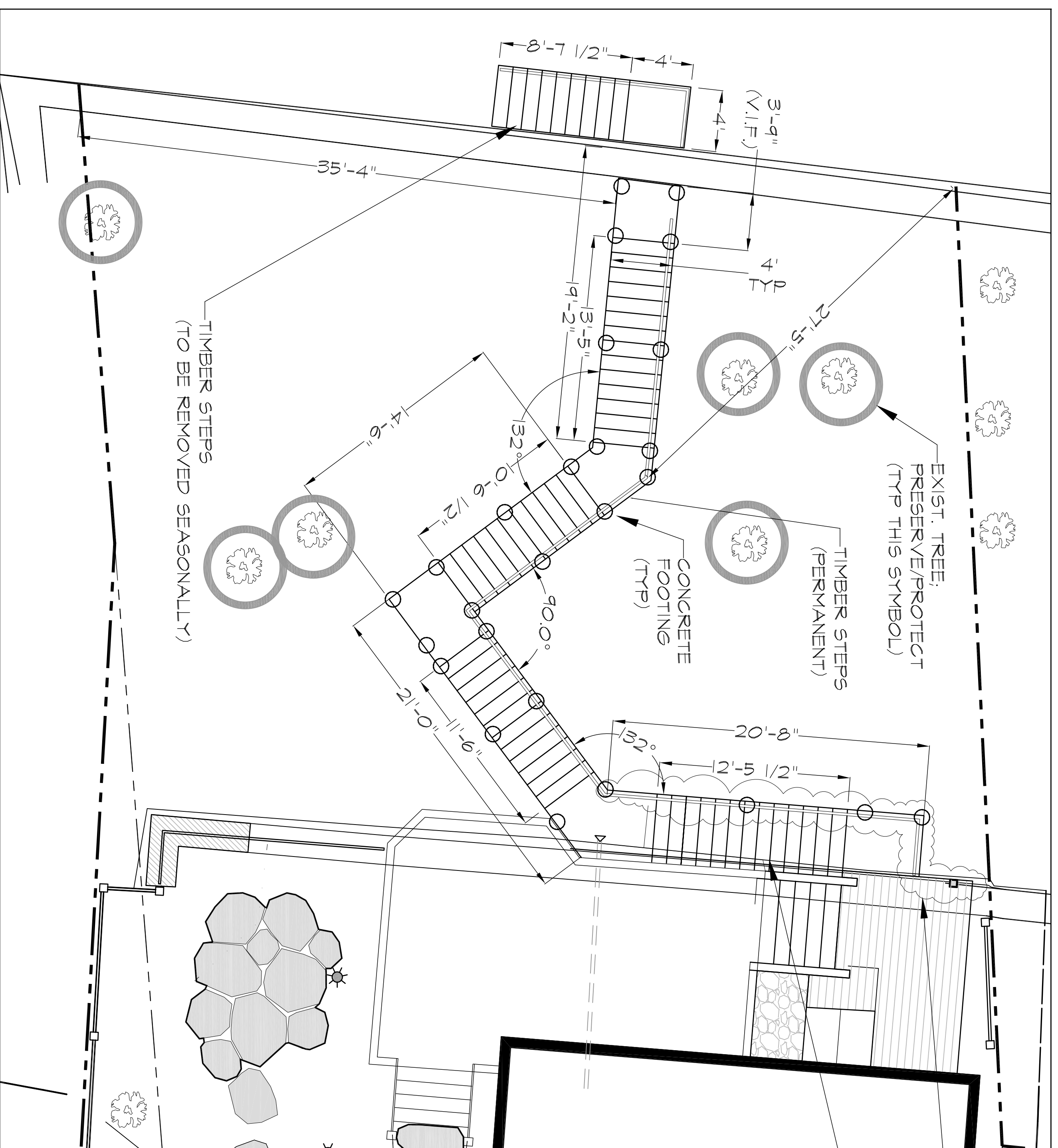
1 TIMBER STEPS - LAYOUT DETAIL NOT TO SCALE
